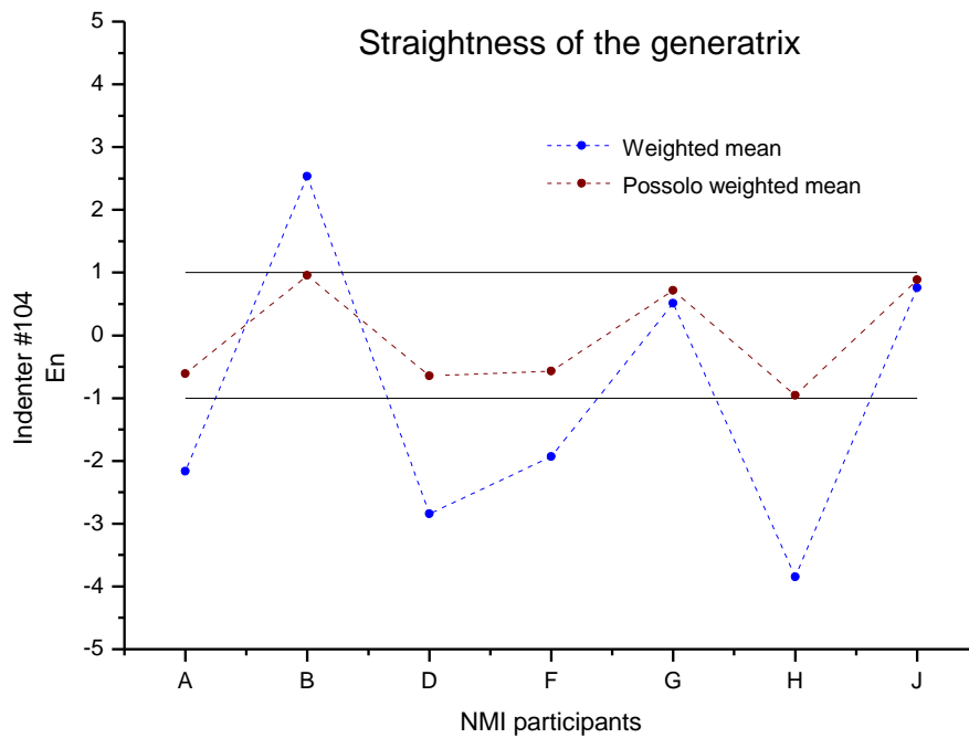
Figure 30: E_n calculated for the NMI participants, related to the straightness of the generatrix of the diamond cone of the indenter #104.
