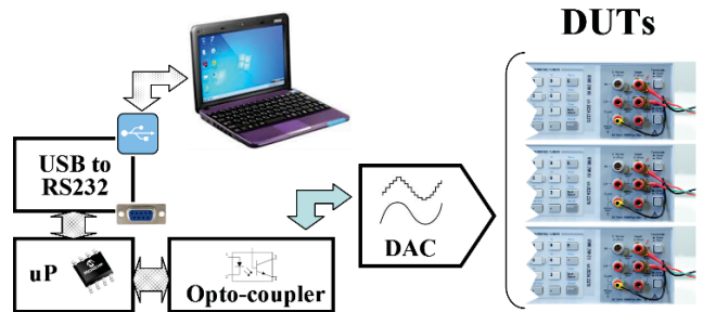
Fig. 5. The control system of the DAC consists of a USB-RS232 converter and a microcontroller, which generates the 16-bit control parameters. The digital part is powered through the computer's USB port. The 16-bit codes are sent serially to two 74LS595 shift registers connected directly to the DAC. The two Bytes stored in the shift registers are dumped with a single clock stroke in the DAC which updates the output voltage. The decoupling of the power supply is achieved by the opto-couplers, placed between the microprocessor and the shift registers. The connection of the DAC to the DMMs takes place with a connection as short as possible and equipped with terminations with low thermo-electromotive forces.
