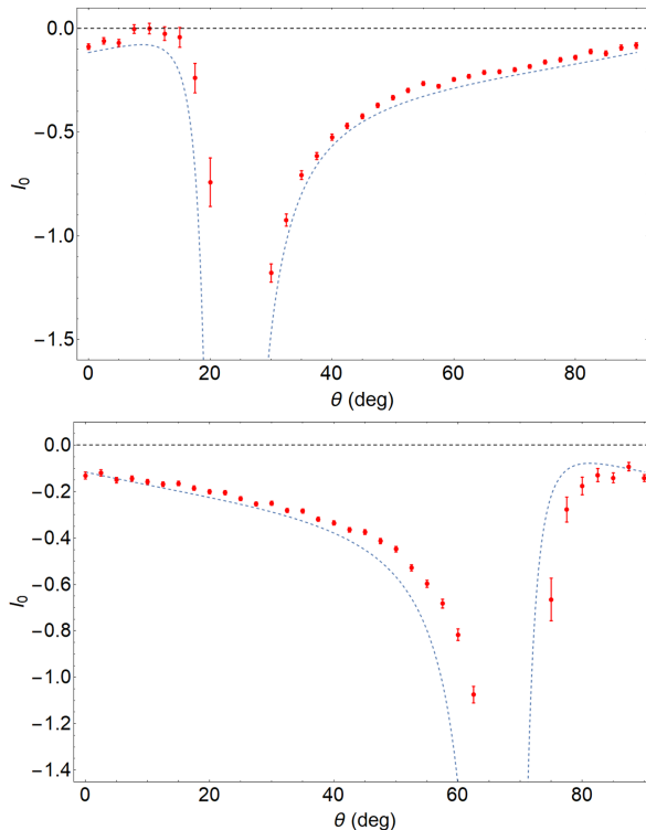
Figure 3. Verification of Pusey inequality for both postselections. The left hand side of inequality (5) is calculated under the best circumstances for disproving the non-contextual model.
