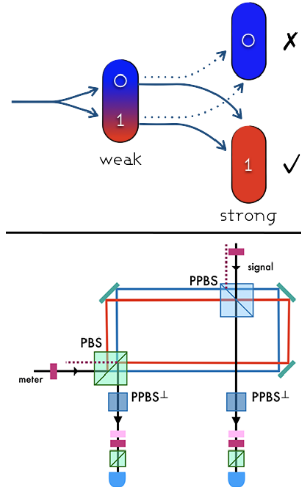
Figure 1. Upper panel: Conceptual scheme. A weak measurement is performed on a qubit with possible outcomes 0 and 1, associated to non-orthogonal states. Events are postselected based on a second strong projective measurement associated to a different observable. Coherent effects are known to give rise to different phenomena. Lower panel: Experimental setup. Signal and meter photons, generated through a Type-I spontaneous parametric down conversion (SPDC) source, are sent through a C-Sign gate [9, 10, 11, 12] implemented within a Sagnac interferometer, as shown. This arrangement benefits from the different paths of the H and V polarized beams (red and blue), which allow to decouple the residual signals (purple dashed lines) given by the imperfect partially polarizing beamsplitter (PPBS) transmission with respect to the measured ones. Two rotated PPBS are used both on the signal and meter to balance polarization losses, and eventually both beams are measured projectively and the coincidence counts are recorded.
