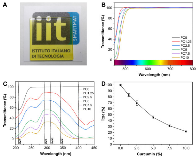
Fig. 4. (A) Photo of PC 10 sample that demonstrates its transparency. (B) Light transmittance ( T\% ) of PC 0, PC 1.25, PC 2.5, PC 5, PC 7.5 and PC 10 in the range 450–800 (Visible range). (C) Light transmittance ( T\% ) of PC 0, PC 1.25, PC 2.5, PC 5, PC 7.5 and PC 10 in the range 200–450 nm (UV range). (D) T_{280} values vs curcumin concentration of PC 0, PC 1.25, PC 2.5, PC 5, PC 7.5 and PC 10.
