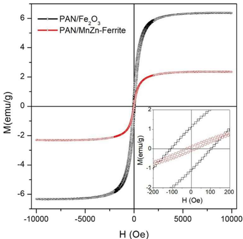
Fig. 7 Room-temperature magnetic hysteresis loops of the PAN/ \text{Fe}_2\text{O}_3 (black squares) and PAN/MnZn-Ferrite (red dots) samples; inset: low magnetic field enlargement
