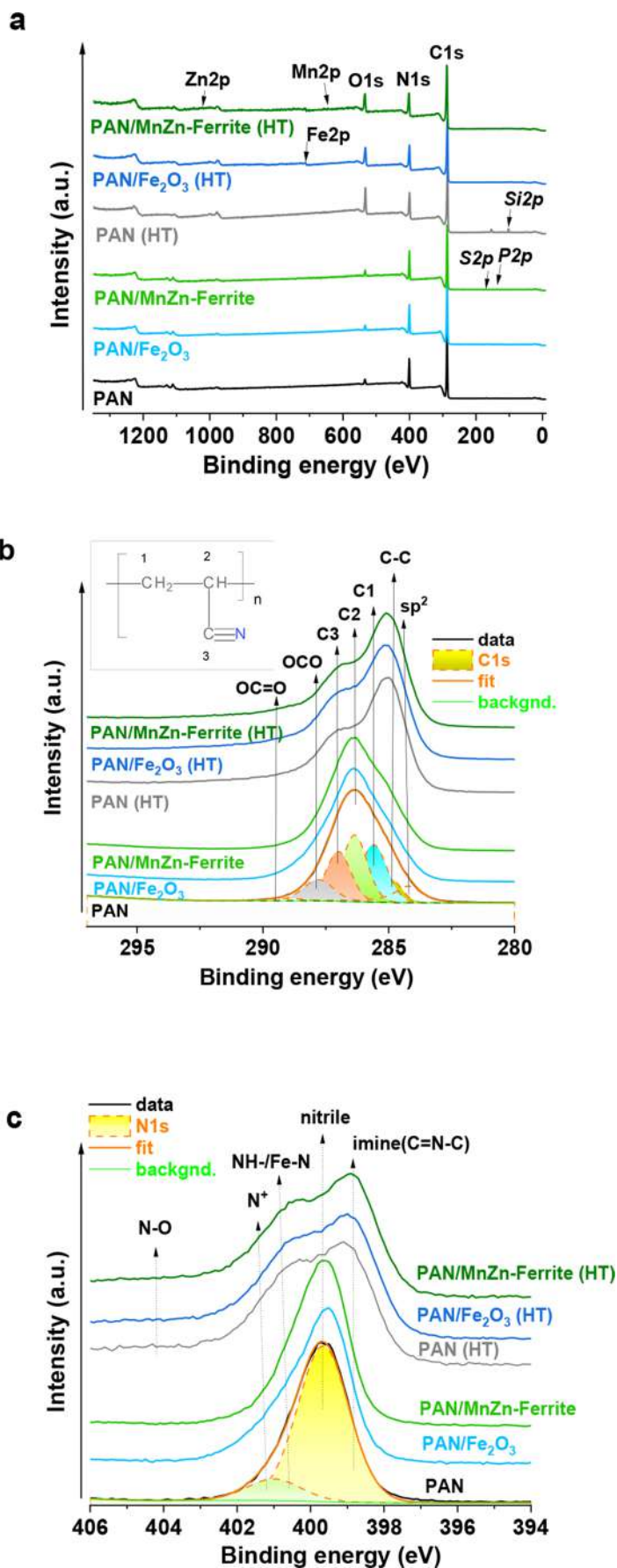
Fig. 5 X-ray photoelectron spectroscopy (a) survey spectrum, (b) C1s and (c) N1s region of PAN, PAN/Fe 2 O 3 and PAN/MnZn-Ferrite before and after heat treatment
