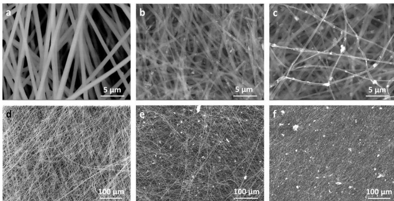
Fig. 2 Enlarged PAN NFs at 20 k \times (a) without nanoparticles, (b) with \gamma -Fe 2 O 3 , (c) with MnZn-Ferrite. PAN NFs at 1000 \times (d) without nanoparticles, (e) with \gamma -Fe 2 O 3 , (f) with MnZn-Ferrite
