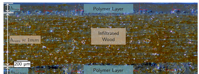
Fig. 1. Cross section of sandwich-type TW samples used for bending tests.
