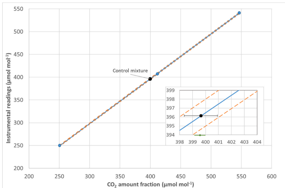
Fig. 2. Example of calibration curve of the NDIR analyser obtained by dynamic dilution in the CO 2 amount fraction range (250–550) μmol·mol −1 . The expanded uncertainty interval ( k = 2 , for a confidence level of approximately 95%) is reported as orange dotted lines. The black dot denotes the control mixture used to validate the calibration curve, while the green dot denotes its certified value. (For interpretation of the references to colour in this figure legend, the reader is referred to the Web version of this article.)
