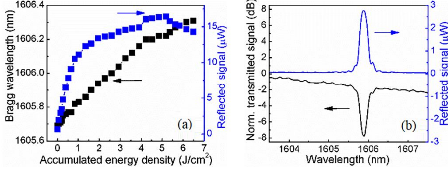
Fig. 9. (a) Bragg wavelength and reflected signal strength evolution during a 100 min inscription of a 5 mm FBG with an UV laser beam pulse energy density of 108 \text{ mJ/cm}^2 and 10 Hz repetition rate. (b) Normalized transmission and reflection signals of a standard FBG after an accumulated energy density dose of 4 \text{ J/cm}^2 . Adapted from [26] under the Creative Common license CC BY.
