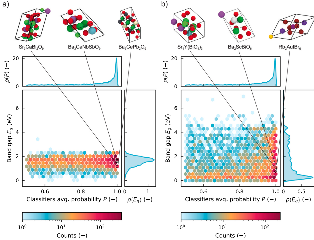
Fig. 4. Hexagonal plot of perovskite candidate materials in the Energy-GNoME database. The hexagon colors represent material counts per region on a logarithmic scale, as indicated by the color bar. Density distributions, \rho , are shown on the plot's top and right, calculated using Gaussian KDE for the average AI-expert probability, P , and the predicted band gap, E_g . For E_g , results are displayed from regressors trained on (a) perovskite data alone and (b) an augmented dataset. The crystal structures above show three notable candidates among the top-ranked perovskite materials, as determined by R^P(y) (see Section 4.6.2). Atom colors follow the extended CPK [47] scheme by Jmol [48]. (For interpretation of the references to color in this figure legend, the reader is referred to the web version of this article.)
