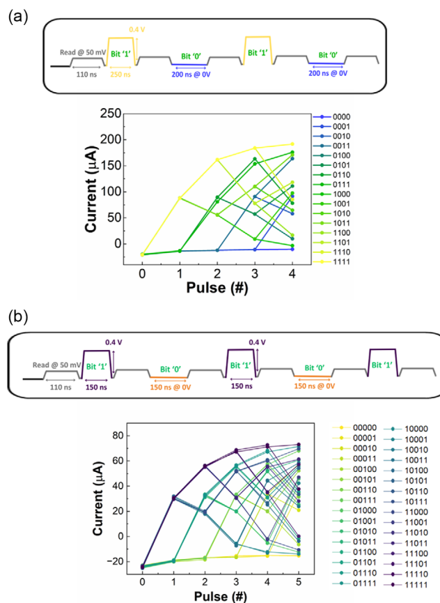
Figure 4. a) Pulse schematic used for 4-bit sequence: bit '1' corresponds to a pulse with 250 ns and 0.4 V and bit '0' corresponds to a 0 V pulse with 200 ns width (mean of ten cycles) and b) pulse schematic used for 5-bit sequence: bit '1' corresponds to a pulse with 150 ns and 0.4 V and bit '0' corresponds to a 0 V pulse with 150 ns width (mean of ten cycles).
