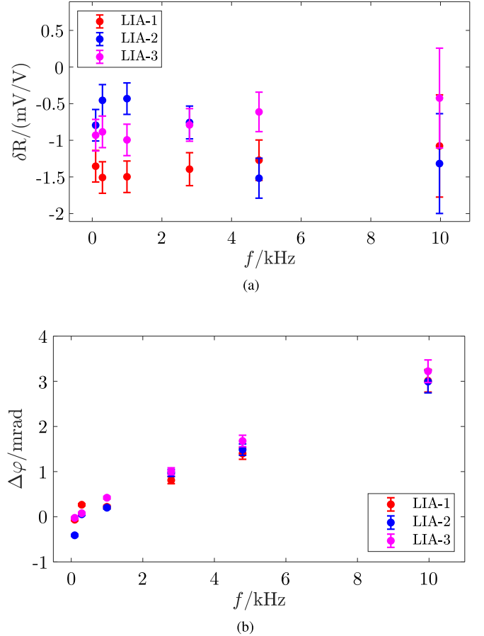
Fig. 3. Comparison of the magnitude and phase calibration of LIA-1 (red), LIA-2 (blue) and LIA-3 (magenta) with |V_{\text{CAL}}^{\text{nom}}| = 5 \mu\text{V} , \varphi_{\text{CAL}}^{\text{nom}} = 45^\circ , and n = 8 , as a function of f_{\text{CAL}} ; LIAs set as per Table III. Uncertainty bars represent combined standard uncertainty. (a) Magnitude error \delta R as a function of f_{\text{CAL}} . (b) Phase error \Delta\varphi as a function of f_{\text{CAL}} .
