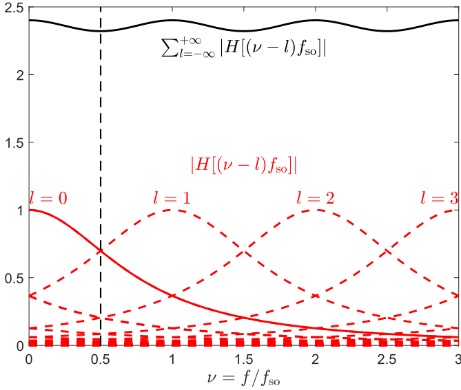
Fig. 7. Transfer functions appearing in the integrand of (17) for n = 1 , T_N = 0.02 s, and f_{SO} \approx 10.46 Hz, parameters for which aliasing is no longer negligible.
