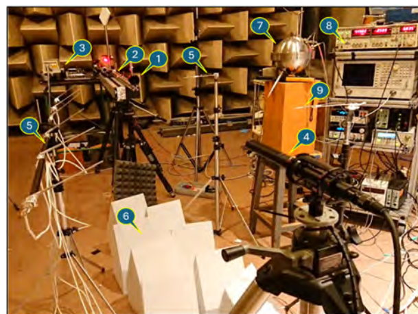
FIG. 10. Experimental setup in a hemi-anechoic chamber for comparison of speed of sound measurements in air with an acoustic wavelength meter and a spherical acoustic resonator. At the background/left is visible the loudspeaker (1) mounted on the moving carriage (2) under the control of an interferometer (3). At the foreground on the right is visible the microphone on the tripod (4). At the left the array of resistance thermometers (5). On the floor foam absorbers for reducing acoustic reflection (6). Top right the spherical resonator (7) with the related electronic bench (8). A hygrometer and a pressure sensor (9), together with a \text{CO}_2 sensor, complete the environmental parameters measurement.
