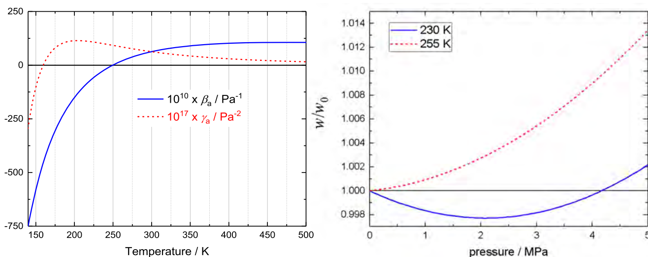
FIG. 5. (Left) Second \beta_a and third \gamma_a acoustic virial pressure coefficient of dry air, respectively showing zero-crossing temperature around 250 and 160 K. (Right) Ratio w/w_0 of speed of sound in dry air to its zero-pressure value for two temperatures: at 230 K the second acoustic virial pressure coefficient \beta_a is negative while the third \gamma_a is positive resulting in a minimum of w around 2 MPa; at 255 K both acoustic virials are positive resulting in a monotonic increasing trend of w . (Right) Ratio w/w_0 of speed of sound in dry air to its zero-pressure value for two temperatures
