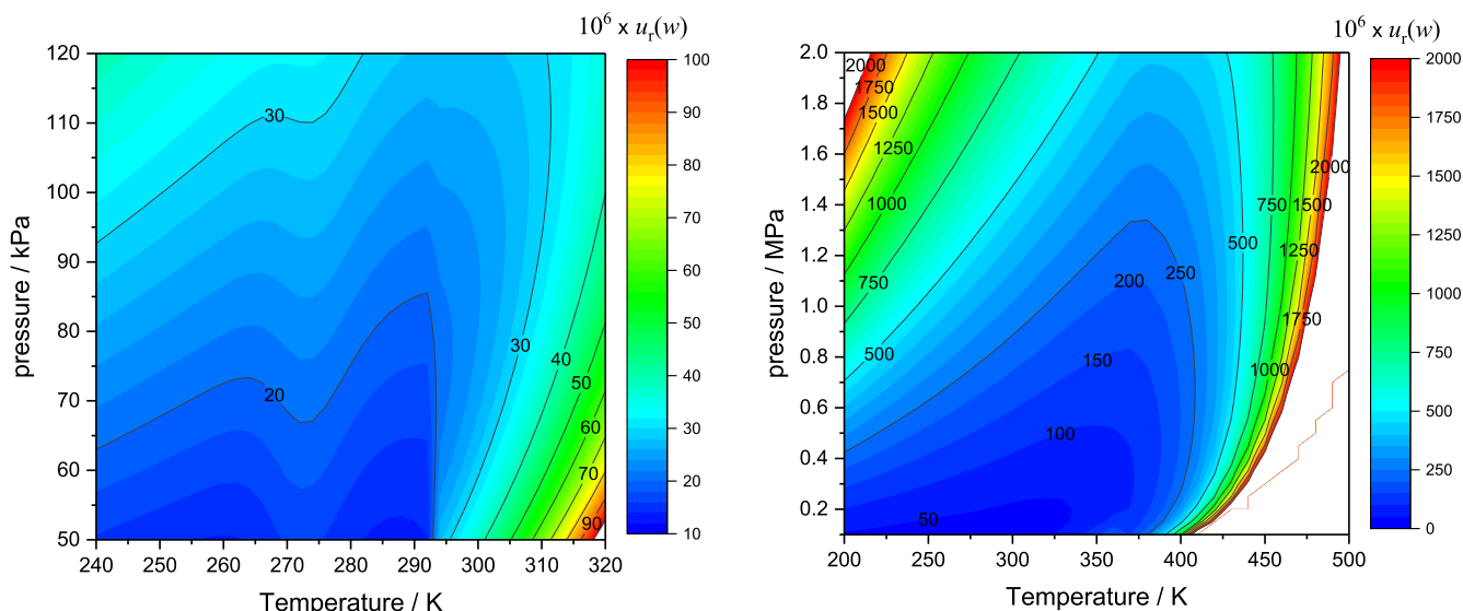
FIG. 9. Relative standard uncertainty of modeled speed of sound in humid air, u_r(w) , as a function of temperature and pressure for a sample of air with h_r = 70\% , x_{CO_2} = 500 ppm, f = 10 kHz. (Left) near-ambient conditions, 240 \text{ K} \leq T \leq 320 \text{ K} , 50 \text{ kPa} \leq p \leq 120 \text{ kPa} . (Right) extended range, 200 \text{ K} \leq T \leq 500 \text{ K} , 100 \text{ kPa} \leq p \leq 2 \text{ MPa} ; white areas correspond to values of u_r(w) exceeding 2000 ppm, and/or combinations p , T resulting in water mole fractions x_w exceeding unity.
