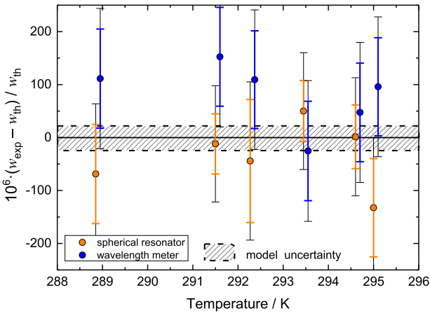
FIG. 21. Relative differences between experimental w_{\text{exp}} and calculated w_{\text{theory}} speed of sound in humid air for a subset of measurements obtained with the wavelength meter (blue) and the spherical resonator (orange). Measurements with the two experiments were corrected to the same reference temperature but are plotted slightly offset on the horizontal axis to facilitate their comparison. Inner (colored) uncertainty bars represent the standard uncertainty of each experiment. Outer (black) uncertainty bars include the uncertainty in the determination of the environmental parameters. The dashed shaded area represents the uncertainty of w_{\text{theory}} .
