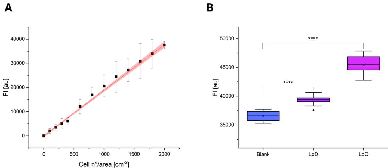
Fig. 2 (A) Estimation of Limits of Blank (LoB), Limits of Detection (LoD), and Limits of Quantification (LoQ) using the calibration curve method. FI_{\text{Sample-Blank}} is plotted on the y-axis against cell concentration on the x-axis, with FI expressed in arbitrary units (au). Error bars represent SD. (B) Experimental validation of LoB, LoD and LoQ, with FI expressed in arbitrary units (au) on y-axis
