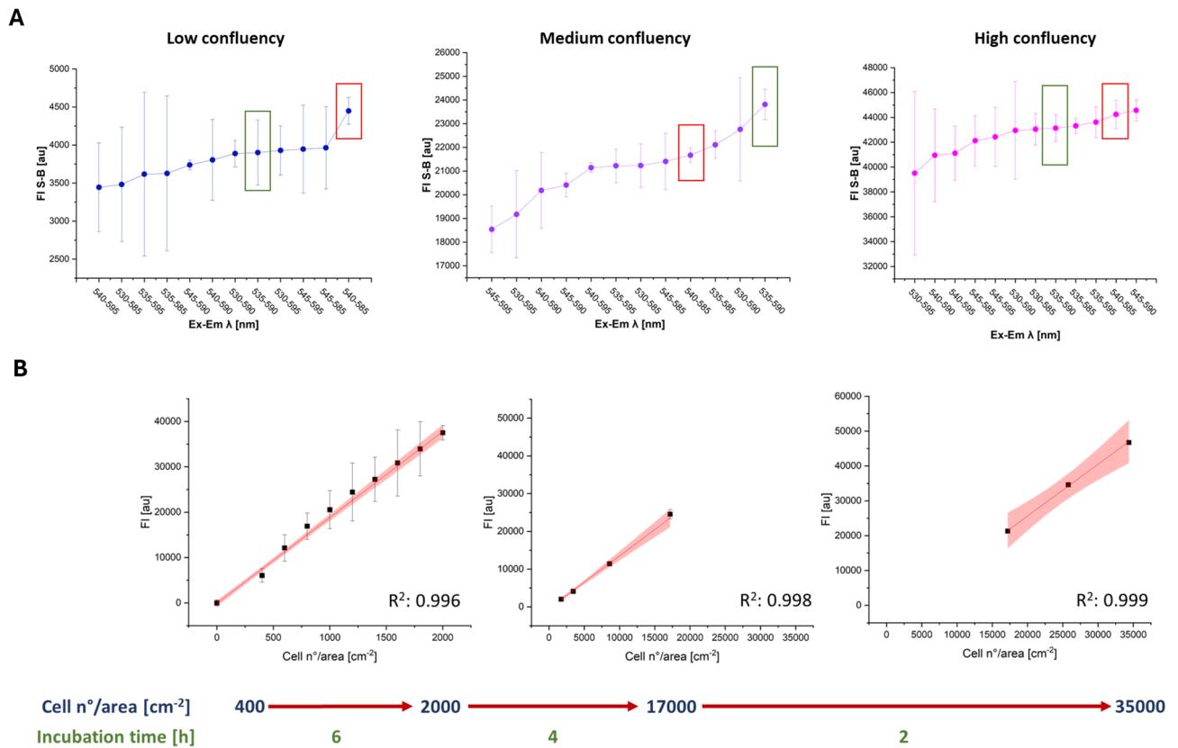
Fig. 1 (A) Fluorescence intensity difference between experimental wells and the Blank sample (FI S-B, y-axis) versus Excitation-Emission wavelengths (Ex-Em \lambda ) combinations (x-axis). FI S-B is expressed in arbitrary units (au); ( \lambda_{Ex} - \lambda_{Em} ) is expressed in nanometers (nm); error bars indicate the standard deviation (SD). The analysis is categorized according to cell confluency levels: low, medium, and high. Two distinct \lambda_{Ex} - \lambda_{Em} combinations have been identified as suitable and are highlighted within boxes: 540–585 nm (red box) and 535–590 nm (green box). (B) FI_{Sample-Blank} (y-axis) plotted against cell concentration (x-axis). Fluorescence intensity (FI) is expressed as arbitrary units (au), and error bars represent standard deviation (SD). Linearity is indicated by R^2 values. The recommended incubation time is indicated in green respect to the cell concentration range (blue)
