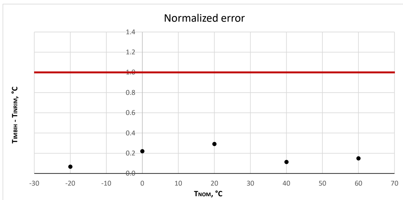
FIGURE 2. NORMALIZED ERROR AT THE CALIBRATION POINTS
