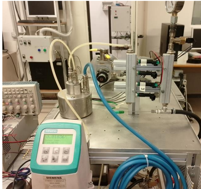
Figure 22: The dynamic hydraulic test bench at UNIPG.
