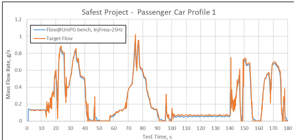
Figure 26: Realization of the Passenger Car Profile 1 with the UNIPG test bench.
