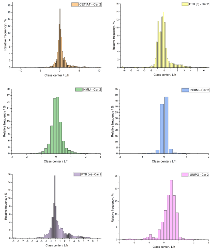
Figure 28: Distribution of residuals passenger car profile 2.
