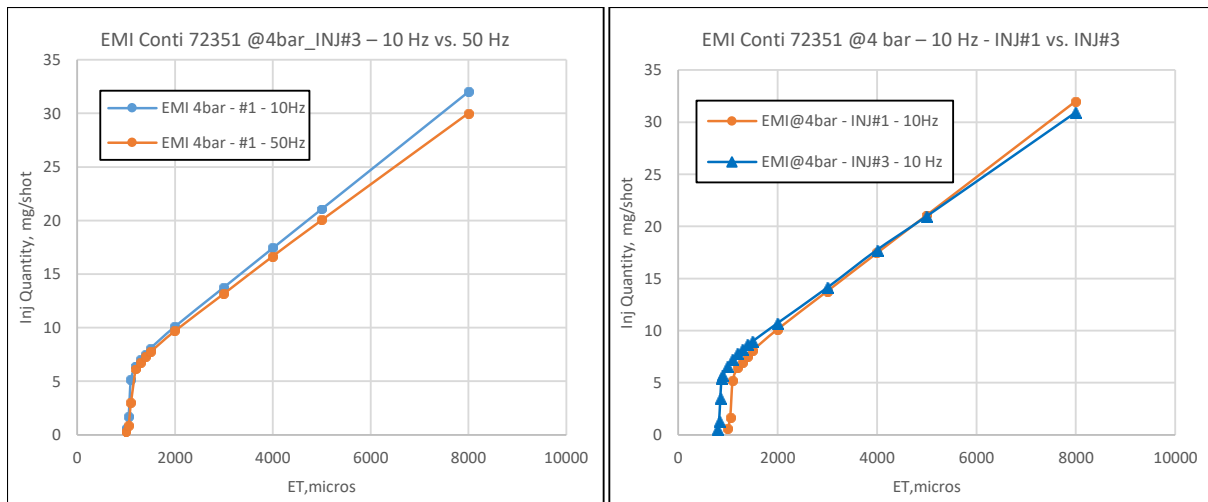
Figure 23: Injector characterization - EMI curves.
