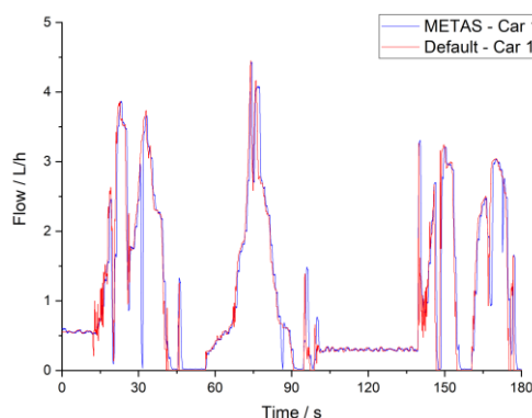
Figure 11: Profile realization METAS.
