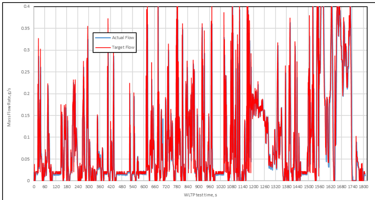
Figure 24: Actual vs. target flow time profiles, obtained with c) strategy.
