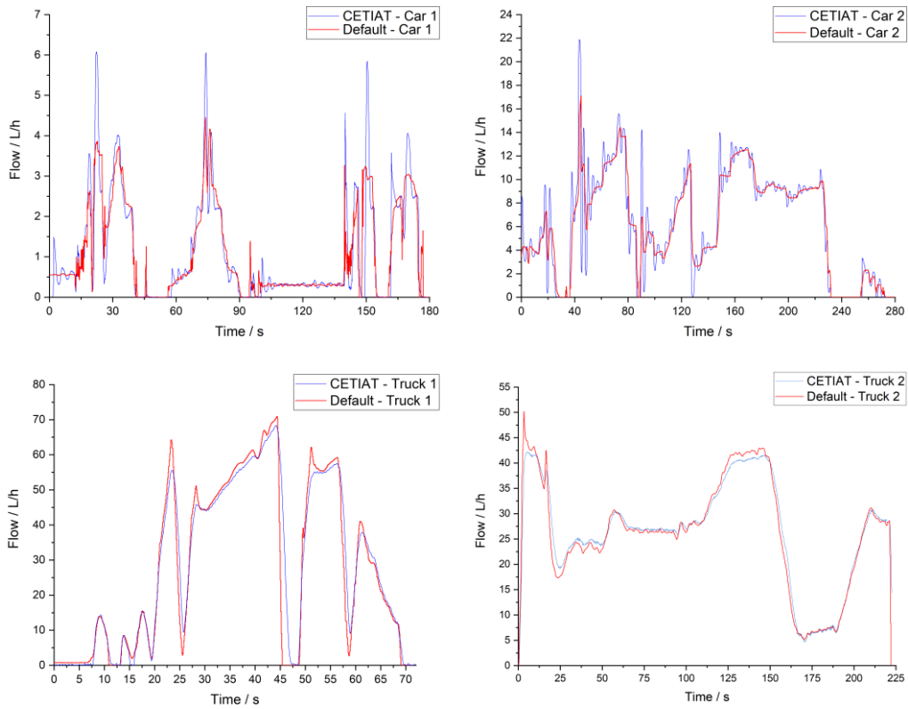
Figure 5: Profile realizations at CETIAT.
