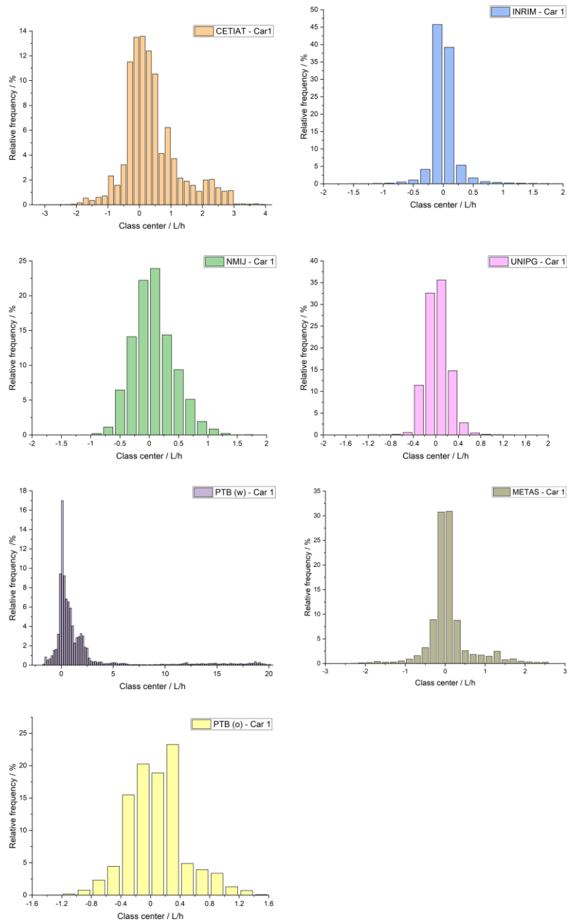
Figure 27: Distribution of residuals for passenger car profile 1.
