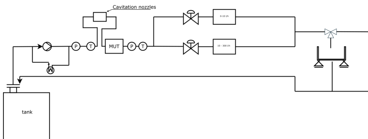
Figure 18: Principal setup of the test bench for measurements using dynamic flow rates at PTB (oil).
