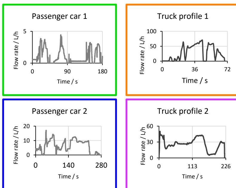
Figure 1: Test profiles used to compare the test benches
