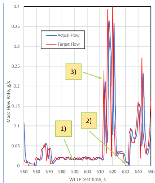
Figure 25: Actual vs. target flow profile obtained with a) strategy; Zoom of Figure 24.
