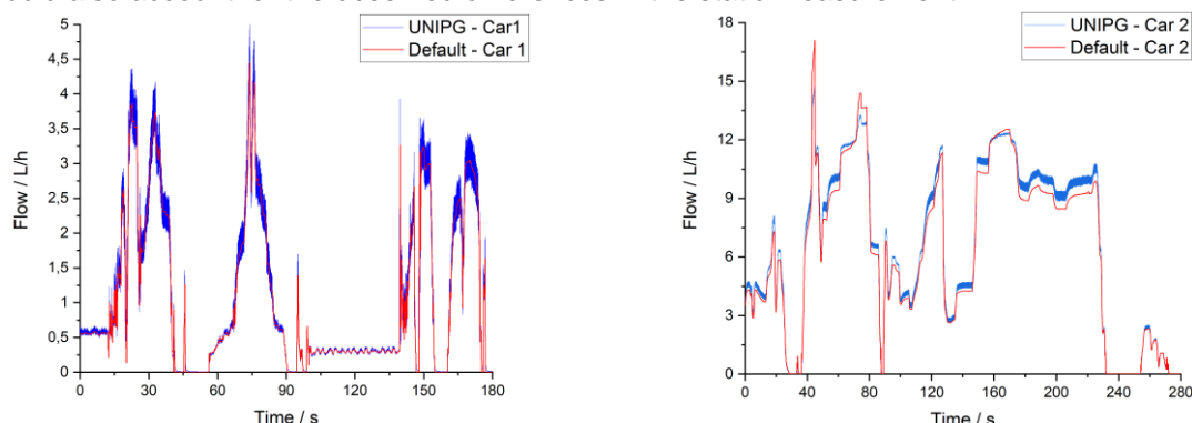
Figure 10: Profile realization UNIPG.
