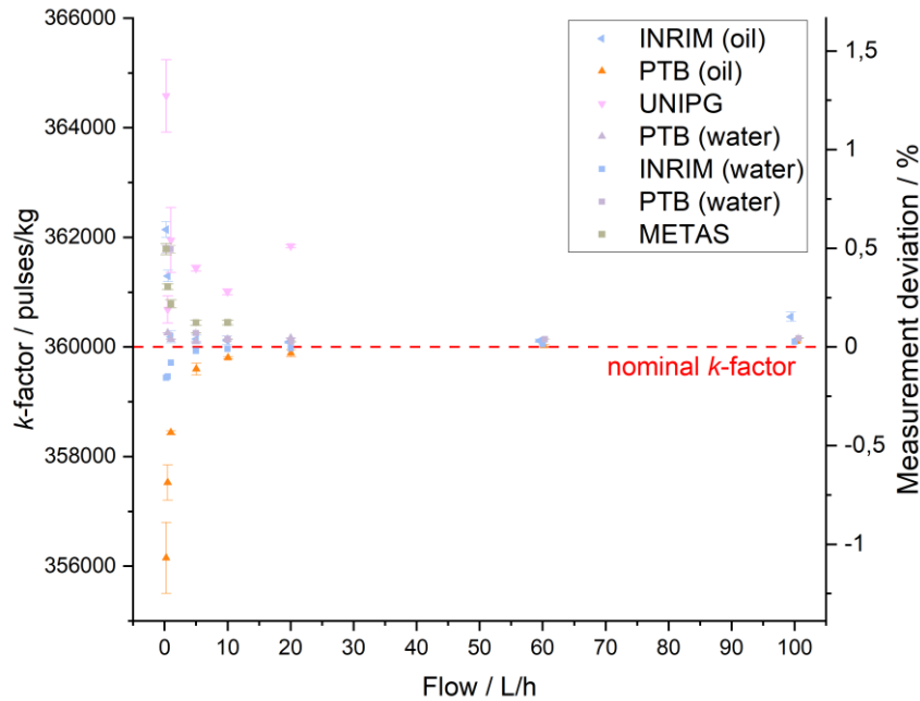
Figure 4: Results of the static measurements (■ water, ▲ calibration oil).
