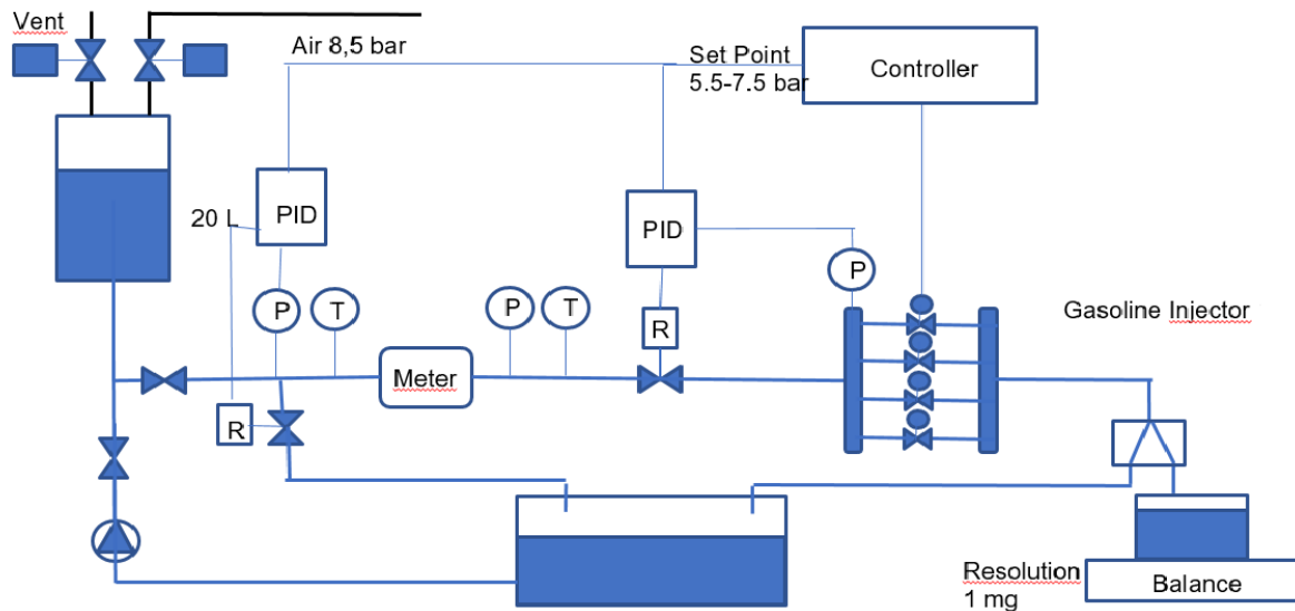
Figure 19: The INRIM test bench for flow meter calibrations.
