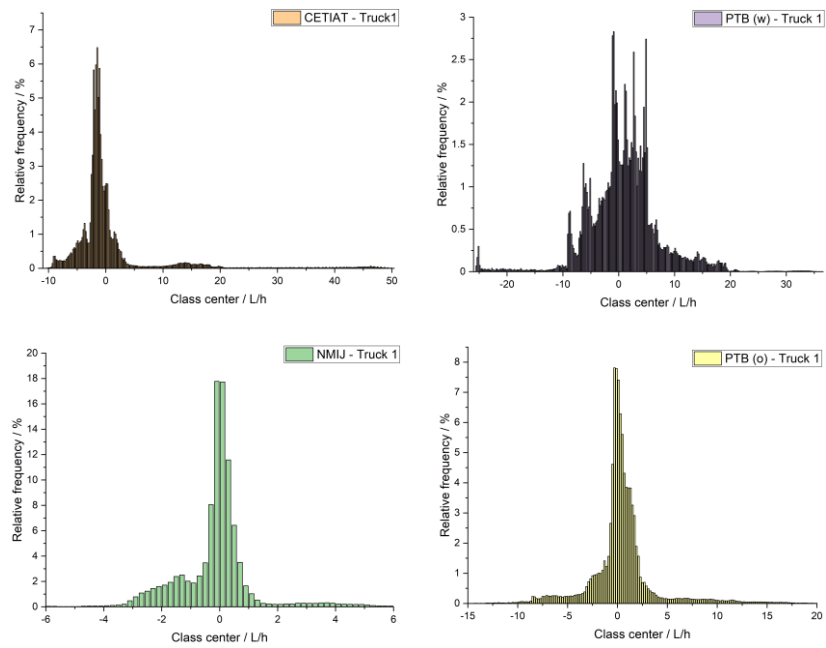
Figure 29: Distribution of residuals truck profile 1.
