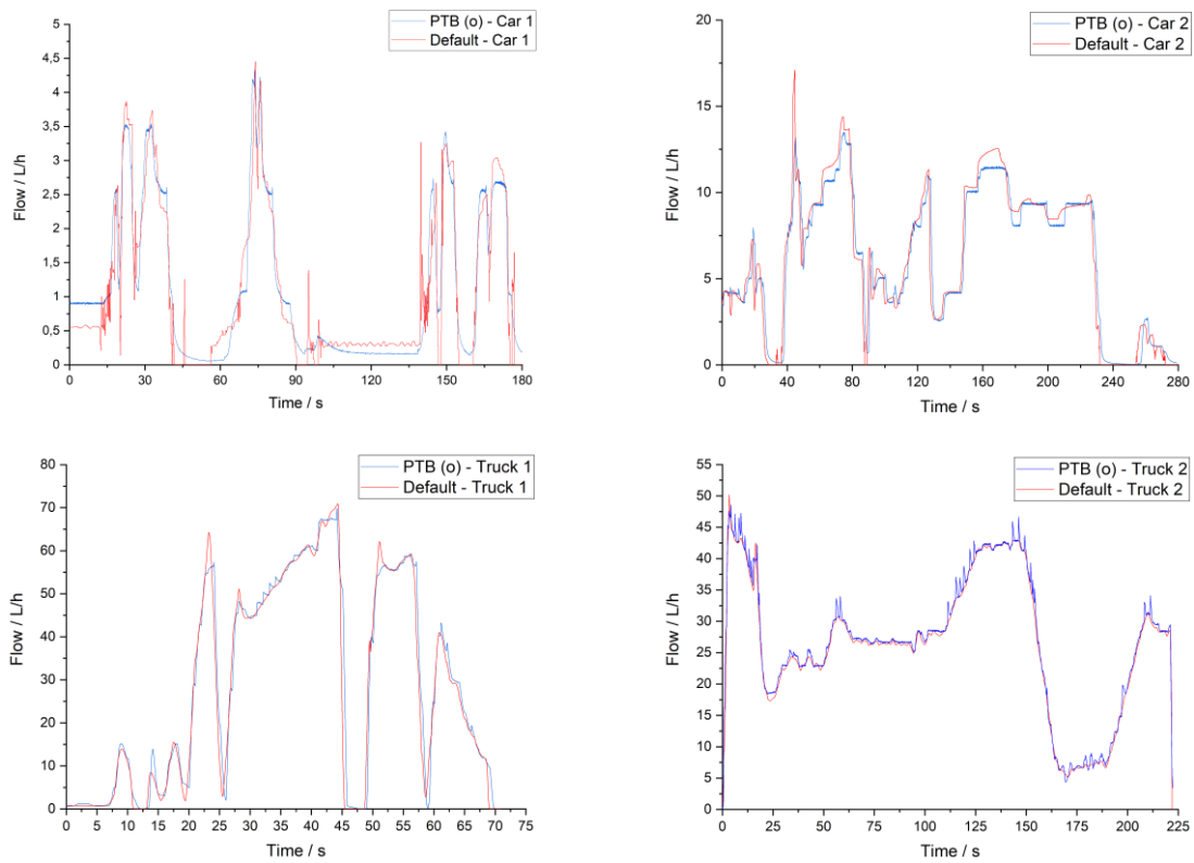
Figure 8: Profile realization PTB oil.
