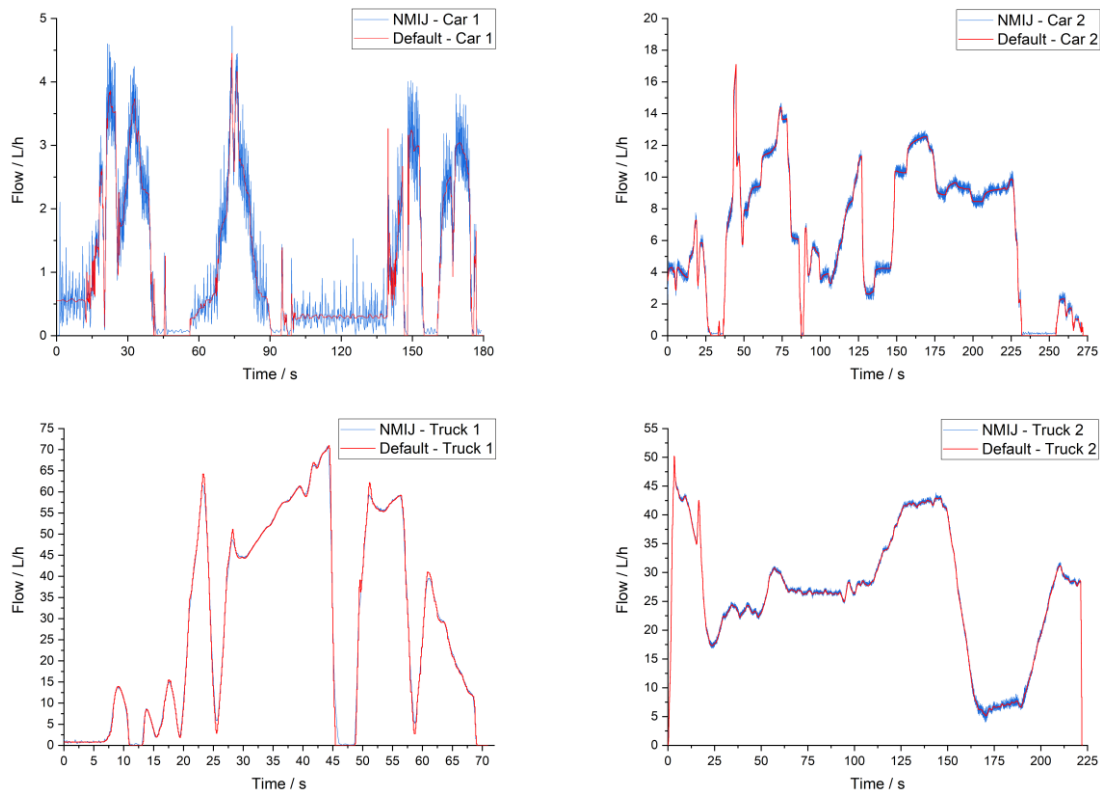
Figure 6: Profile realization NMIJ.
