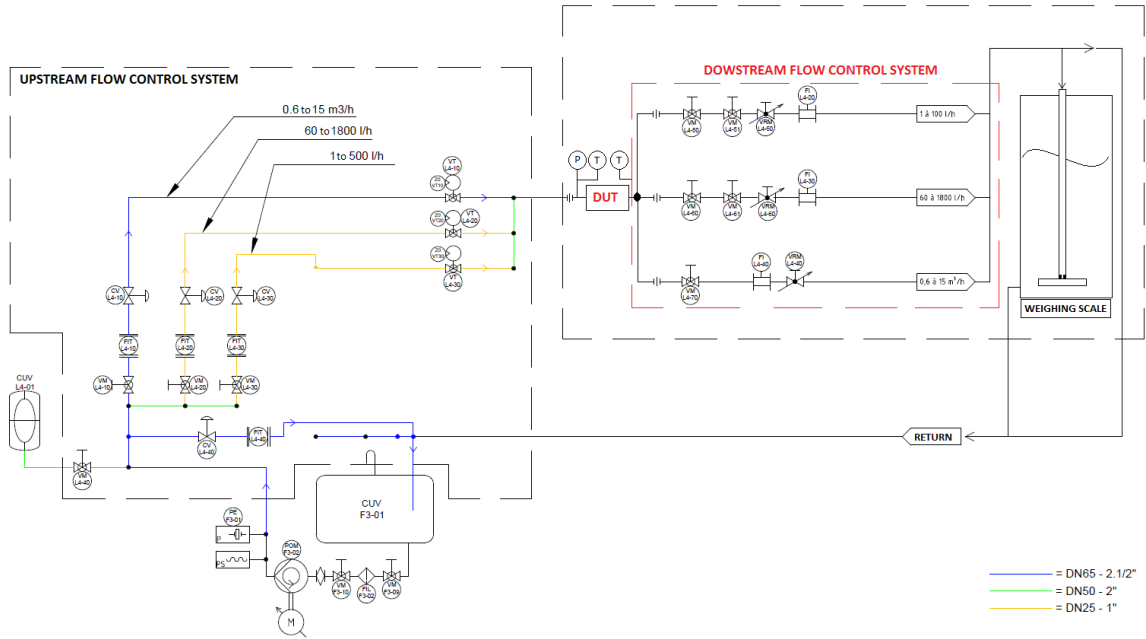
Figure 16: Schematic of Cetiats dynamic test bench.
