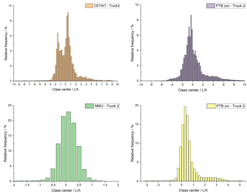
Figure 30: Distribution of residuals truck profile 2.
