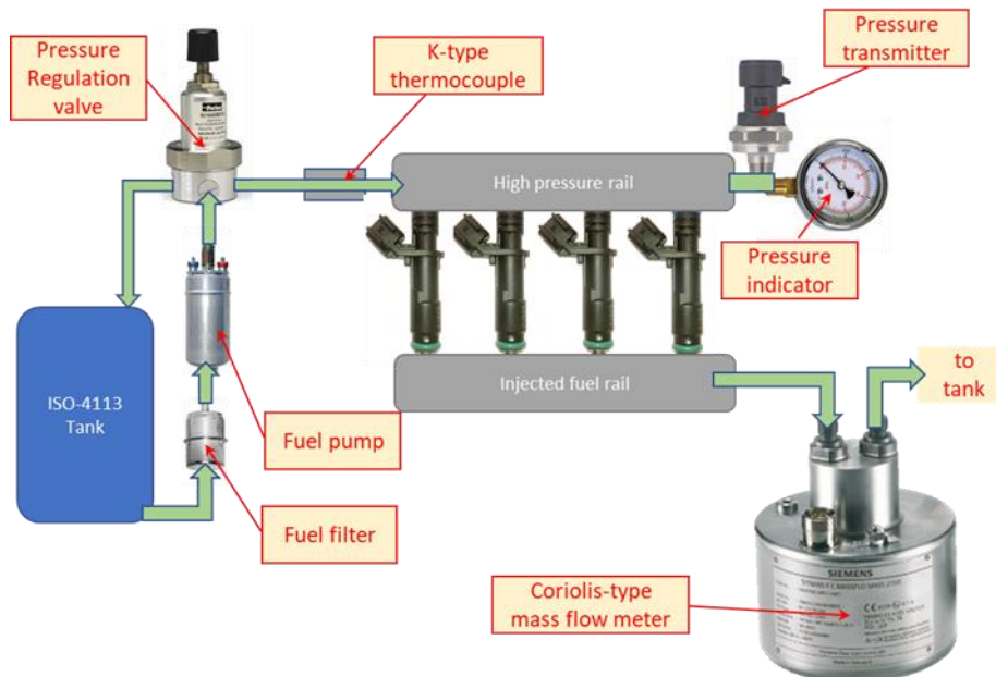
Figure 21: Schematic of the Dynamic Hydraulic Test Bench used.
