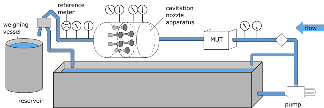
Figure 17: Principal setup of the test bench for measurements using dynamic flow rates at PTB (water).
