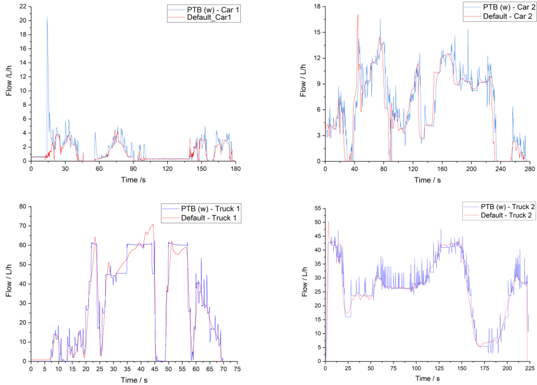
Figure 7: Profile realization PTB water.
