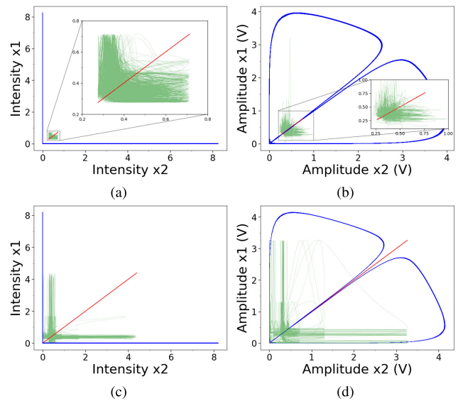
FIGURE 8. Synchronization of chaos as a function of coupling strength \epsilon . Numerical integration (left panels): (a) synchronization of SC in phase space x_1 - x_2 ; (c) synchronization of HC in phase space x_1 - x_2 . Spice simulation (right panels): (b) synchronization of SC in phase space x_1 - x_2 ; (d) synchronization of HC in phase space x_1 - x_2 .
