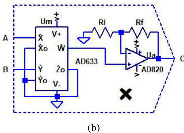
FIGURE 2. (a) Schematic of the circuit implementing the minimal universal model. (b) Structure of a single nonlinear block, having two input ports A , B and an output port C .
