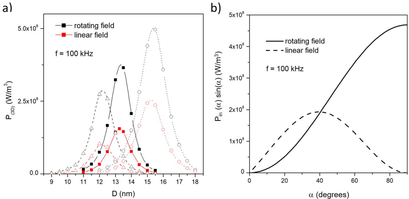
FIG. 8. a) intrinsic power density P_{(3D)} of magnetite nanoparticles of different size with easy axes randomly distributed in space and submitted to a rotating field with H_V = 100 Oe (black lines and symbols); the same quantity obtained using a field of same frequency and amplitude directed along the x -axis (red lines and symbols); full squares/full line: size-independent magnetic properties of particles; open circles/dotted lines: size-dependent properties (case a) of the Appendix; open triangles/dashed lines: size-dependent properties (case b) of the Appendix; b) behaviour of the \alpha -dependent power density for nanoparticles submitted to the rotating and to the linear field (full/dashed lines).
