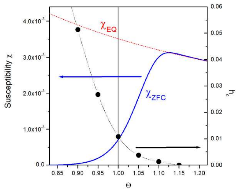
Figure 3: Coercive field h_c (symbols), ZFC susceptibility \chi_{ZFC} (blue full line) and equilibrium susceptibility \chi_{EQ} (red dotted line) around blocking temperature for collinear monodisperse nanoparticles ( \phi = 0 ).
