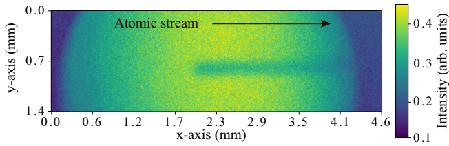
FIG. 10. Atomic fluorescence in the cavity seen through a cavity mirror. We couple a 689 nm beam into the cavity. This addresses the atoms at the center of the cavity, roughly 2 mm along the x axis, where they are transferred to |e\rangle , transparent to the fluorescence beam. The cut is chosen to highlight the dark stripe due to these flying atoms.
