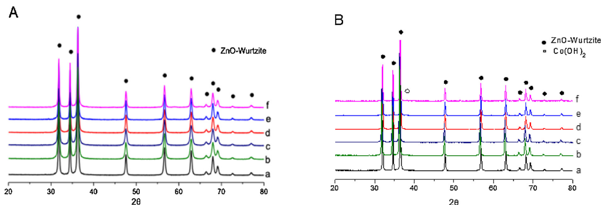
Fig. 1. Diffratograms of bare and Co-ZnO prepared via (A) solution and (B) hydrothermal methods, a) pristine ZnO, b) Co(0.25%)-ZnO, c) Co(0.5%)-ZnO, d) Co(1%)-ZnO, e) Co(3%)-ZnO, f) Co(5%)-ZnO.
