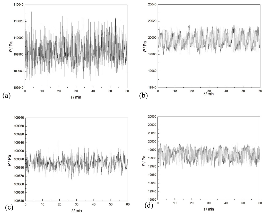
Figure 2. Pressure stability under the following nominal conditions: (a) \phi = 4 \text{ l}\cdot\text{min}^{-1} , p = 1100 \text{ hPa} and T_{\text{sat}} = -99.3^\circ\text{C} . Peak-to-peak amplitude = 0.92 hPa, mean value = 1099.85 hPa, standard deviation = 17 Pa; (b) \phi = 1.5 \text{ l}\cdot\text{min}^{-1} , p = 200 \text{ hPa} and T_{\text{sat}} = -99.3^\circ\text{C} . Peak-to-peak amplitude = 0.39 hPa, mean value = 199.97 hPa, standard deviation = 8 Pa; (c) \phi = 5 \text{ l}\cdot\text{min}^{-1} , p = 1100 \text{ hPa} and T_{\text{sat}} = -75^\circ\text{C} . Peak-to-peak amplitude = 0.64 hPa, mean value = 1098.86 hPa, standard deviation = 7 Pa; (d) \phi = 1.5 \text{ l}\cdot\text{min}^{-1} , p = 200 \text{ hPa} and T_{\text{sat}} = -75^\circ\text{C} . Peak-to-peak amplitude = 0.35 hPa, mean value = 199.85 hPa, standard deviation = 7 Pa. All flow rates are at pressure.
