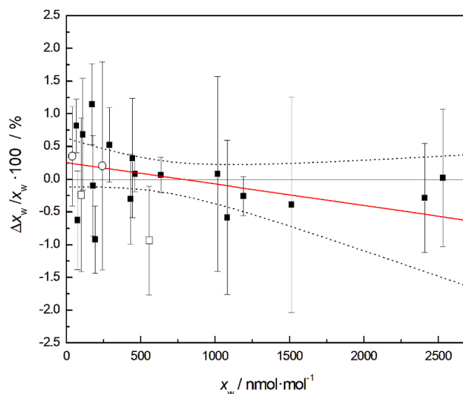
Figure 12. Percentage relative differences 100 \cdot \Delta x_w/x_w , as a function of x_w , between the water vapour amount fraction as measured before and after the heating of the generator outlet pipe (■); before and after the increase and decrease of T_{\text{sat}} (○); before and after the decrease and increase of T_{\text{sat}} (□). The estimated coefficients of the linear regression equation \Delta x_w/x_w = a + b \cdot x_w and their standard uncertainties are: a = (0.26 \pm 0.18) and b = (-3.28 \pm 2.20) \cdot 10^{-4} \text{ nmol}^{-1} \cdot \text{mol} . Regression line (—). Upper and lower 95% confidence limits (---).
