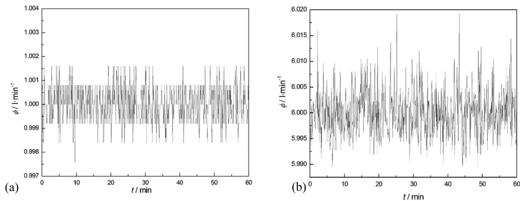
Figure 3. Flow rate stability under the following nominal conditions: (a) \phi = 1 \text{ l}\cdot\text{min}^{-1} , p = 200 \text{ hPa} and T_{\text{sat}} = -99^\circ\text{C} . Peak-to-peak amplitude = 5.6 \text{ml}\cdot\text{min}^{-1} , mean value = 1.000 \text{l}\cdot\text{min}^{-1} , standard deviation = 0.8 \text{ml}\cdot\text{min}^{-1} . (b) \phi = 6 \text{ l}\cdot\text{min}^{-1} , p = 1100 \text{ hPa} and T_{\text{sat}} = -94^\circ\text{C} . Peak-to-peak amplitude = 33.6 \text{ml}\cdot\text{min}^{-1} , mean value = 6.00 \text{l}\cdot\text{min}^{-1} , standard deviation = 4.6 \text{ml}\cdot\text{min}^{-1} . Flow rates are at pressure.
