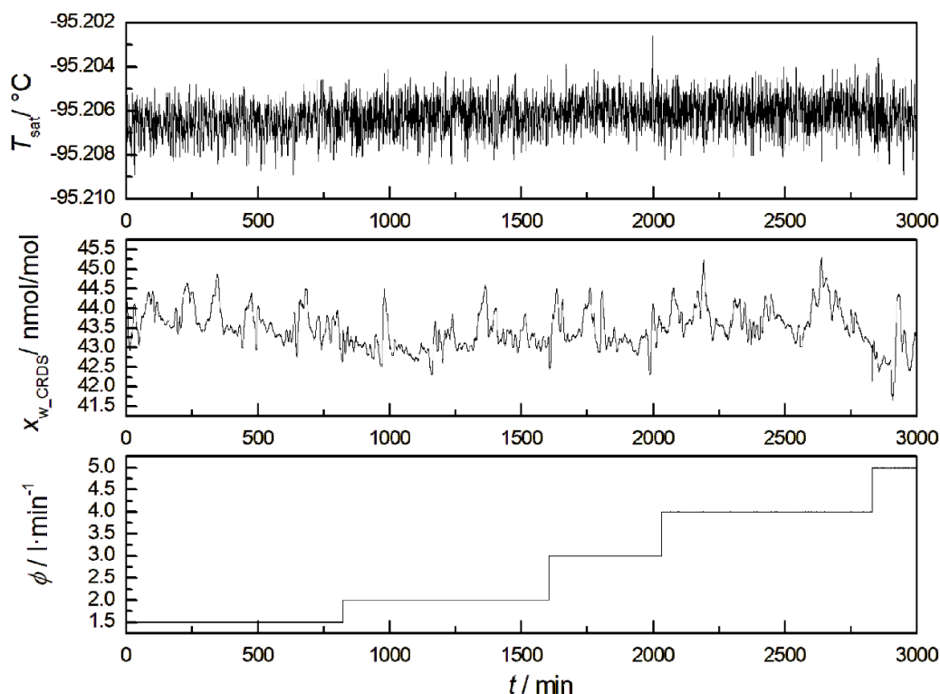
Figure 5. Water vapour amount fraction as measured by the CRDS, x_{w\_CRDS} , as a function of the flow rate, \phi , that ranges between 1.5 and 5 l min -1 at operating pressure. The saturation temperature, T_{sat} is shown in the same time interval. The experiment was carried out at an absolute gas pressure of 800 hPa.
