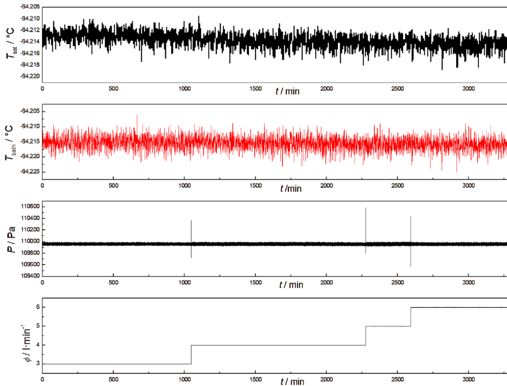
Figure 4. Stability of the water vapour saturation temperature T_{\text{sat}} and saturator bath temperature T_{\text{bath}} at a nominal temperature of -94\text{ }^{\circ}\text{C} , pressure of 1100 hPa and flow rate \phi between 3 and 6 \text{l}\cdot\text{min}^{-1} . The temperature difference between T_{\text{sat}} and T_{\text{bath}} is lower than 3 mK.
