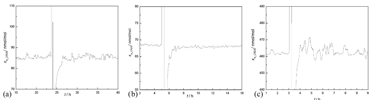
Figure 10. Adsorption/desorption effects of water vapour on the inner surface of the generator outlet EP-SS tubing detected through the measurement of the water vapour amount fraction, x_{w,CRDS} , before and after heating the outlet pipe, in the following conditions: (a) T_{sat} = -99\text{ }^{\circ}\text{C} , p = 200\text{ hPa} , \phi = 1.5\text{ l}\cdot\text{min}^{-1} ; (b) T_{sat} = -94\text{ }^{\circ}\text{C} , p = 500\text{ hPa} , \phi = 2\text{ l}\cdot\text{min}^{-1} ; (c) T_{sat} = -80\text{ }^{\circ}\text{C} , p = 1100\text{ hPa} , \phi = 2\text{ l}\cdot\text{min}^{-1} .
