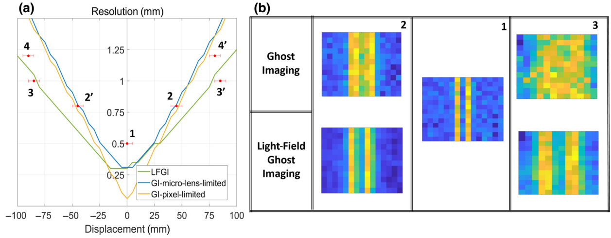
FIG. 3. Resolution of GI and LFGI as a function of the displacement. (a) The curves represent the set of points where the visibility of a double slit is exactly 40% for the GI-microlens-limited, GI-pixel-limited, and LFGI reconstructions, respectively. (b) Examples of GI and LFGI reconstructions of double-slit masks with different separations and different displacements, as indicated by the red circles in (a). The same conclusions can be derived from the other points (“2’,” “3’,” “4,” “4’”) that are not reported for brevity. All LFGI reconstructions show visibility greater than or equal to 40%.
