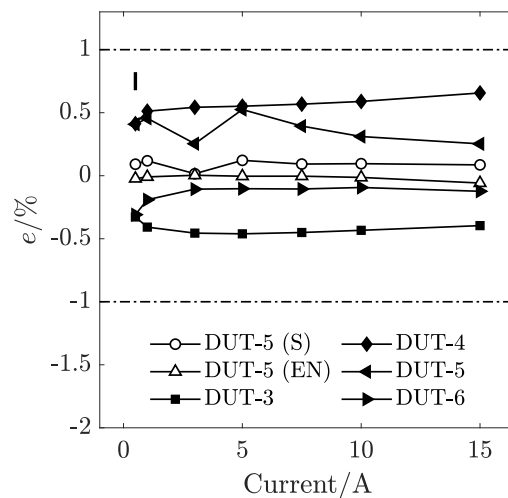
Figure 6. Relative error, e , between W_{REF} and W_{DUT} for measurements performed with DUT-3 to DUT-6. Black markers represent the error on the measurement of reproduced distorted waveforms; white circles correspond to sinusoidal conditions and white triangles to the standardised distorted conditions, labeled as (S) and (EN) respectively in the legend, here reported as a reference for DUT-5 only for sake of clarity. The horizontal dashed lines indicate the accuracy class of the DUTs according to EN 50470; the vertical marker represents the worst combined uncertainty among all the measurements, equal to 0.072%.
