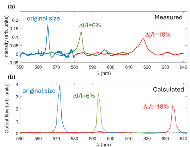
FIG. 5. (a) Measured transmission spectra of guided BSW from scaled cavities: original pattern (blue line); scaled cavity with \Delta l/l = 6\% (green line), scaled cavity with \Delta l/l = 18\% (red line); (b) Calculated output flow from the waveguide: original pattern (blue dashed line), scaled cavity with \Delta l/l = 6\% (green dashed line), scaled cavity with \Delta l/l = 18\% (red dashed line).
