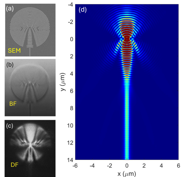
FIG. 3. Images of a fabricated cavity taken with (a) scanning electron microscope and optical microscope in (b) bright field and (c) dark field, respectively. The DF image is collected in a no-BSW coupling condition. (d) Intensity distribution ( |E(x, y)|^2 ) of light emitted by a dipole in the cavity center and coupled within the waveguide. The colormap is thresholded such that the intensity at the source location is at saturation.
