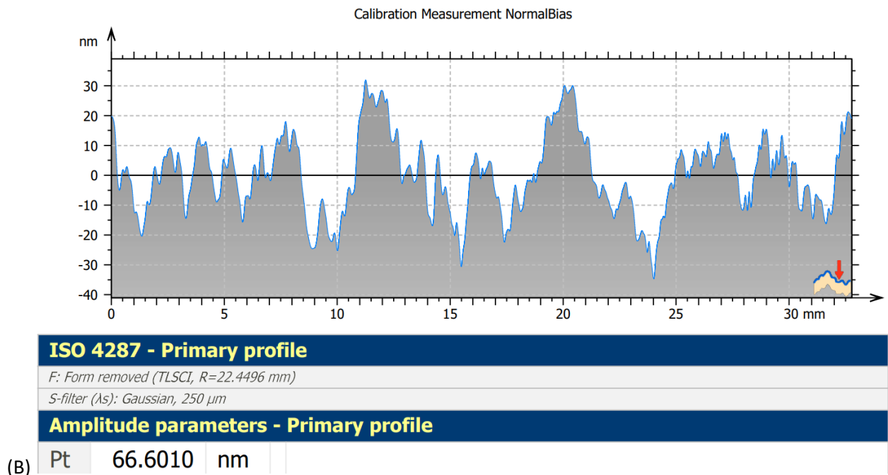
FIGURE 6 – (A) PRECISION CERAMIC SPHERE CALIBRATED AT INRiM AND (B) ITS PROFILE AND Pt
