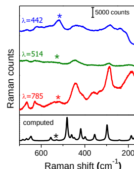
Figure 4. Ce-O cluster vibrational modes region of Raman spectra of Ce-UiO-66-ADC acquired with different \lambda_{\text{inc}} . Black line: computed spectrum.
