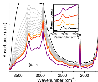
Figure 2. FT-IR spectra collected during Ce-UiO-66-ADC thermal activation. Inset: Raman spectra reported in the 2400-1900 cm -1 (triple bonds stretching region) range collected with \lambda_{\text{inc}} = 785 nm. Black: as synthesized RT; grey: in vacuum RT outgassing; yellow: 30°C; orange: 60°C; violet: 90°C.
