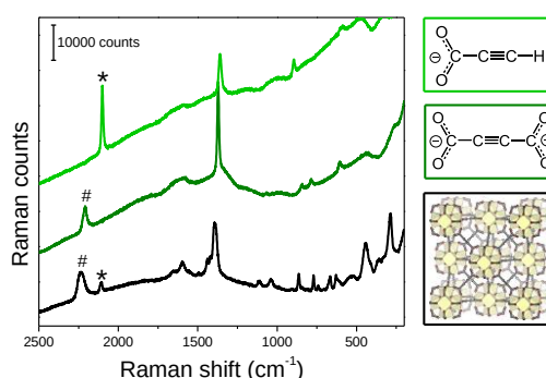
Figure 3. Raman spectra ( \lambda_{\text{inc}} = 785 nm) of: Ce-UiO-66-ADC (black), acetylene dicarboxylate solution (dark green), propiolate solution (light green).
