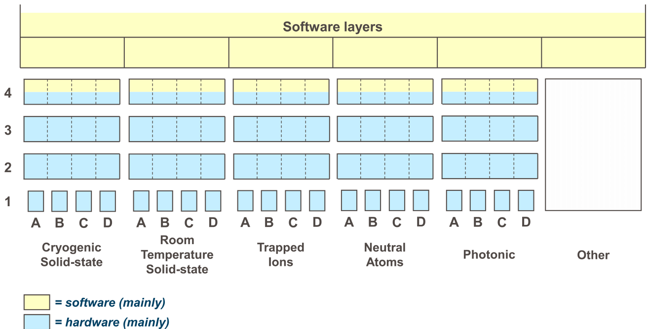
Figure 11 A possible break-down of quantum computing into layered stacks, accounting for different architectures
