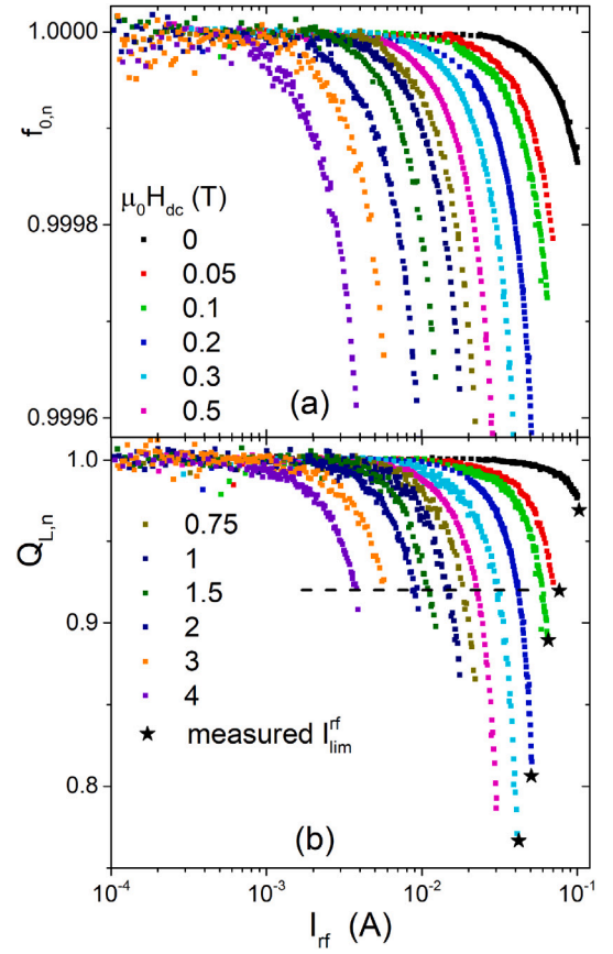
Fig. 4. (a) Resonance frequency normalized by its low-power value, as a function of the rf current circulating in the CPWR at the resonance, for different values of applied dc magnetic field. (b) Normalized unloaded quality factor. Star symbols indicate limiting rf current values, obtained as the maximum current just before jump occurrence in the resonance curves. The black dashed line was used to determine the shifts in I_{lim}^{rf} as a function of dc field, when jumps were not observed.
