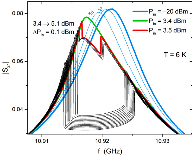
Fig. 2. CPWR resonance curves measured for different values of input rf power, P_{in} , from the linear regime to the nonlinear one. Reference curves are highlighted, corresponding to: -20 dB m input power (linear regime); +3.4 dB m and +3.5 dB m, just before and after the first weak link switching.
