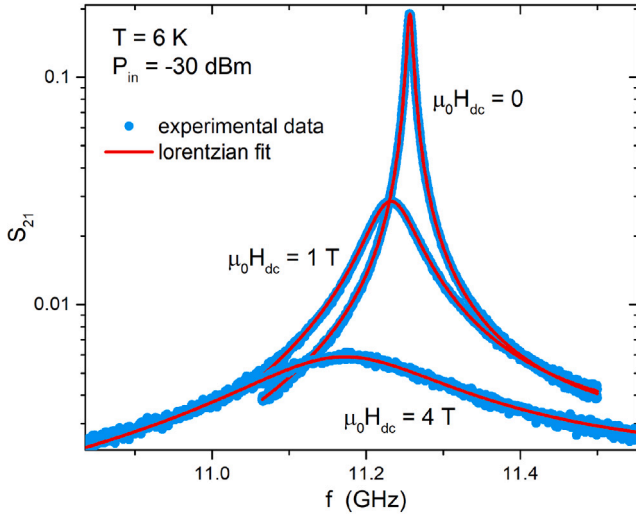
Fig. 1. Resonance curves for different values of dc magnetic field, from 0 to 4 T, in the low rf-power linear regime. Experimental data are fitted by the function reported in Eq. (1).
