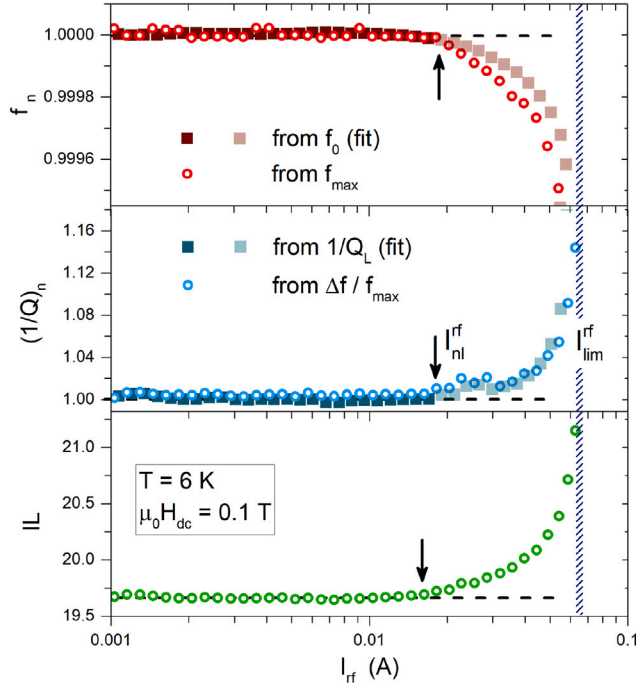
Fig. 3. Resonance frequency, normalized by its low-power value (a), inverse of the loaded quality factor, normalized by its low-power value (b), and insertion loss (c) as a function of the rf current circulating in the CPWR at the resonance, calculated by Eq. (2). Data were extracted from Lorentzian fits of the resonance curves ( f_0 , Q_L ) and directly from the experimental S_{21}(T) resonance curves (frequency at the maximum, f_{max} , curve width at -3 dB, \Delta f ), insertion loss IL = -20\text{Log}(|S_{21}|^{max}) . The limiting rf current I_{lim}^{rf} is the maximum current flowing in the CPWR.
