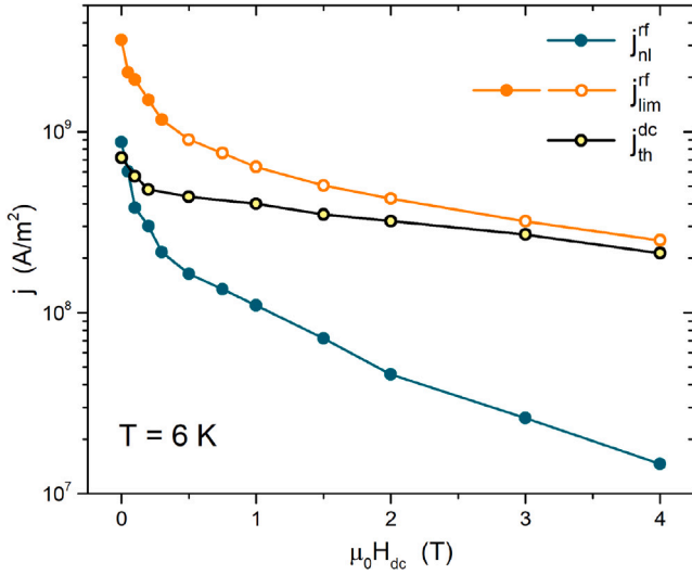
Fig. 5. Comparison among the reference current densities discussed throughout the text: j_{ni}^{rf} is the threshold current density above which nonlinearities emerge; j_{lim}^{rf} is the limiting rf current density (solid symbols: data measured in the presence of a jump, open symbols: extrapolated data, see main text); j_{th}^{dc} indicates the onset of dissipation in current-voltage dc characteristics.
