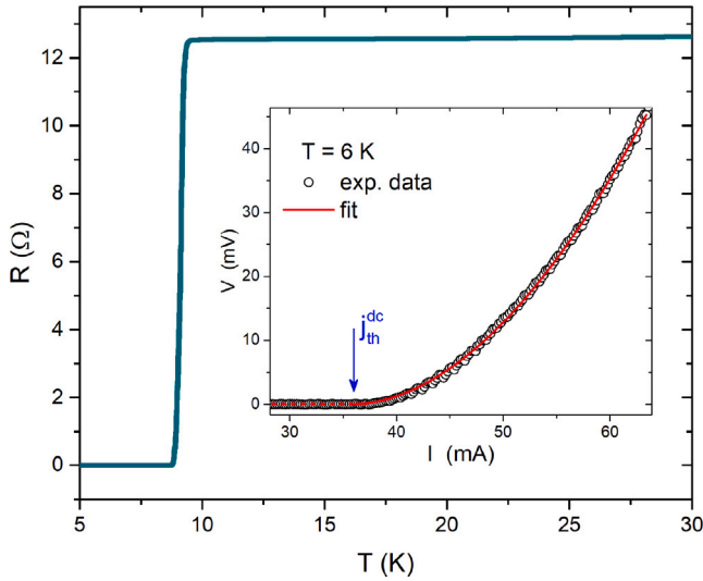
Fig. 6. Dc resistance vs. temperature curve of a NbTi Hall bar, at zero field. In the inset, a current-voltage curve is reported at the temperature of 6 K and for an applied dc magnetic field of 1 T. The fit to a flux creep model is shown (see text for details) and the onset of dissipation j_{th}^{dc} is indicated by an arrow.
