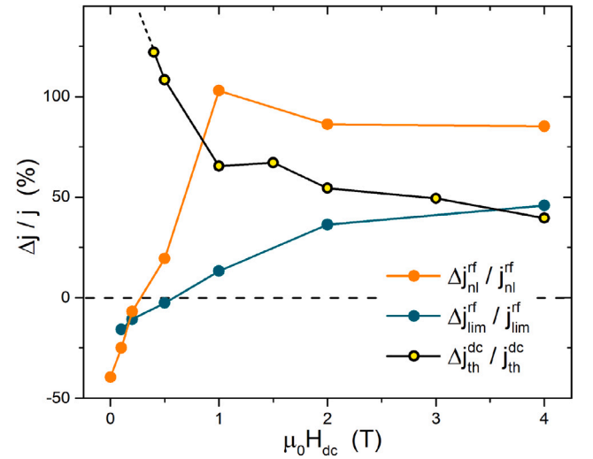
Fig. 8. Effects of proton irradiation on the reference current densities, at T = 6 K, as a function of dc applied field: percentage variation of the nonlinearity threshold current density j_{nl}^{rf} , of the limiting current density j_{lim}^{rf} , and of the dc current density at the onset of dissipation, j_{th}^{dc} . The same CPWR and Hall bar were measured before and after irradiation. The dotted line at the dc curve indicates that at low field the increment is undefined but surely higher than 100% (we measured the current density before irradiation, but after irradiation we could not because the critical current was higher than 100 mA, which is the limit of our apparatus).
