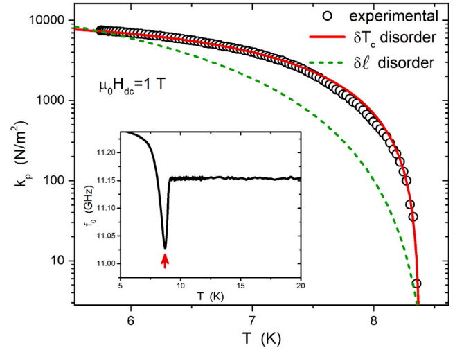
Fig. 7. Pinning constant k_p as a function of temperature, for an applied dc field of 1 T. The red line is the behavior expected for \delta T_c pinning, according to Eq. (5), while the green dashed line shows what would be the temperature dependence in the case of \delta \ell pinning. In the inset, the observed f_0(T) anomaly is reported. (For interpretation of the references to color in this figure legend, the reader is referred to the web version of this article.)
