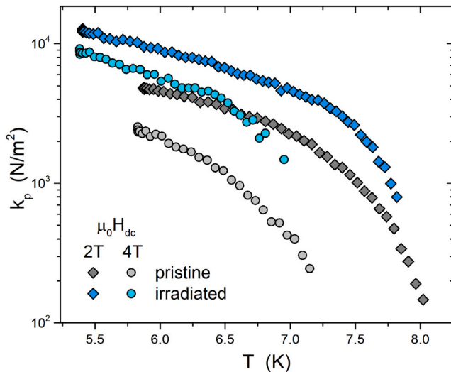
Fig. 9. Pinning constant as a function of temperature for different applied magnetic fields, for the same CPWR before and after proton irradiation.
