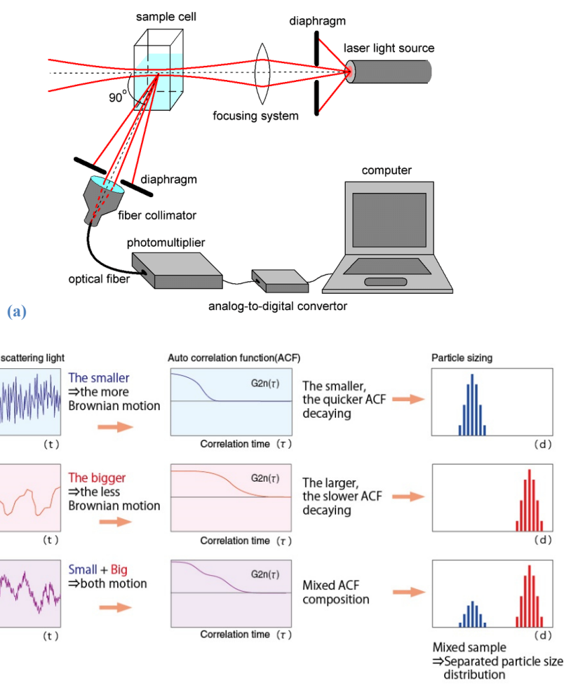
Figure 1. 8 (a) Scheme of a Dynamic Light Scattering (DLS) spectrometer.
