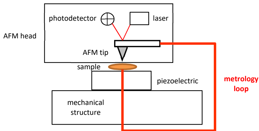
Figure 2. 10 Example of a metrology loop for an AFM.
