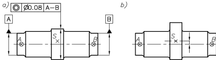
Fig. 2. Characteristic points for the measurement model of coaxiality: a) drawing with characteristic points, b) visualization of the deviation
