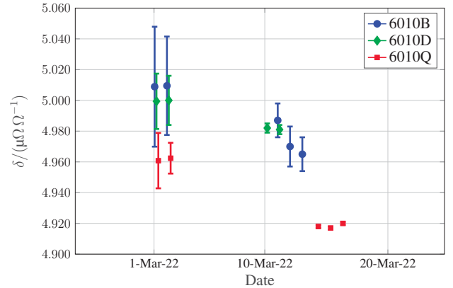
Fig. 1. 10/1 ratio. Relative deviations from the nominal ratio 10/1 for different measurements performed in about 20 days with the 6010B (blue), the 6010D (green) and 6010Q (red).
