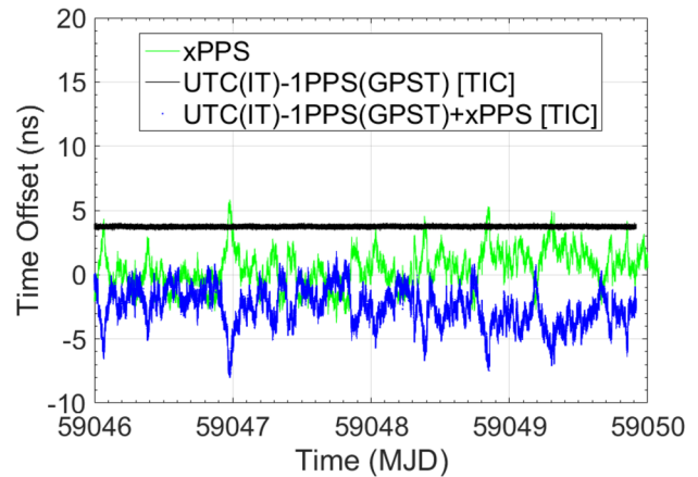
Fig. 5 INR6 in UTC(IT) referenced mode of operation and SYS DLY applied at receiver level. Improved stability in the TIC measurements and absence of cycle slips are depictable
