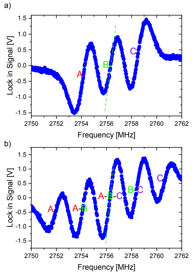
Fig. 4. Lock-in spectrum of an ensemble of NV centers. (a) Single frequency excitation, the linear regions labelled with letters A, B, C corresponds to the dips in Fig. 1 (b) Simultaneous Hyperfine driving, exciting simultaneously with three frequencies, all the three dips are excited when the center frequency corresponds to the central dips, and hence the slope of the curve is enhanced
