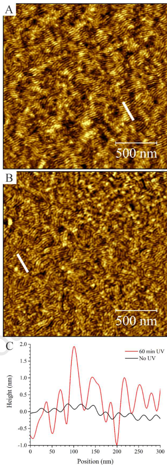
Figure 3. AFM height images of PS- b -PMMA thin films, prepared by spin coating toluene solutions of 1 wt% BCP onto ITO-FSM6 supports after thermal annealing at 190 °C for 24 hours, before (A) and after (B) 60 min of UV irradiation. Height profiles extracted from the AFM micrographs are reported in C.
