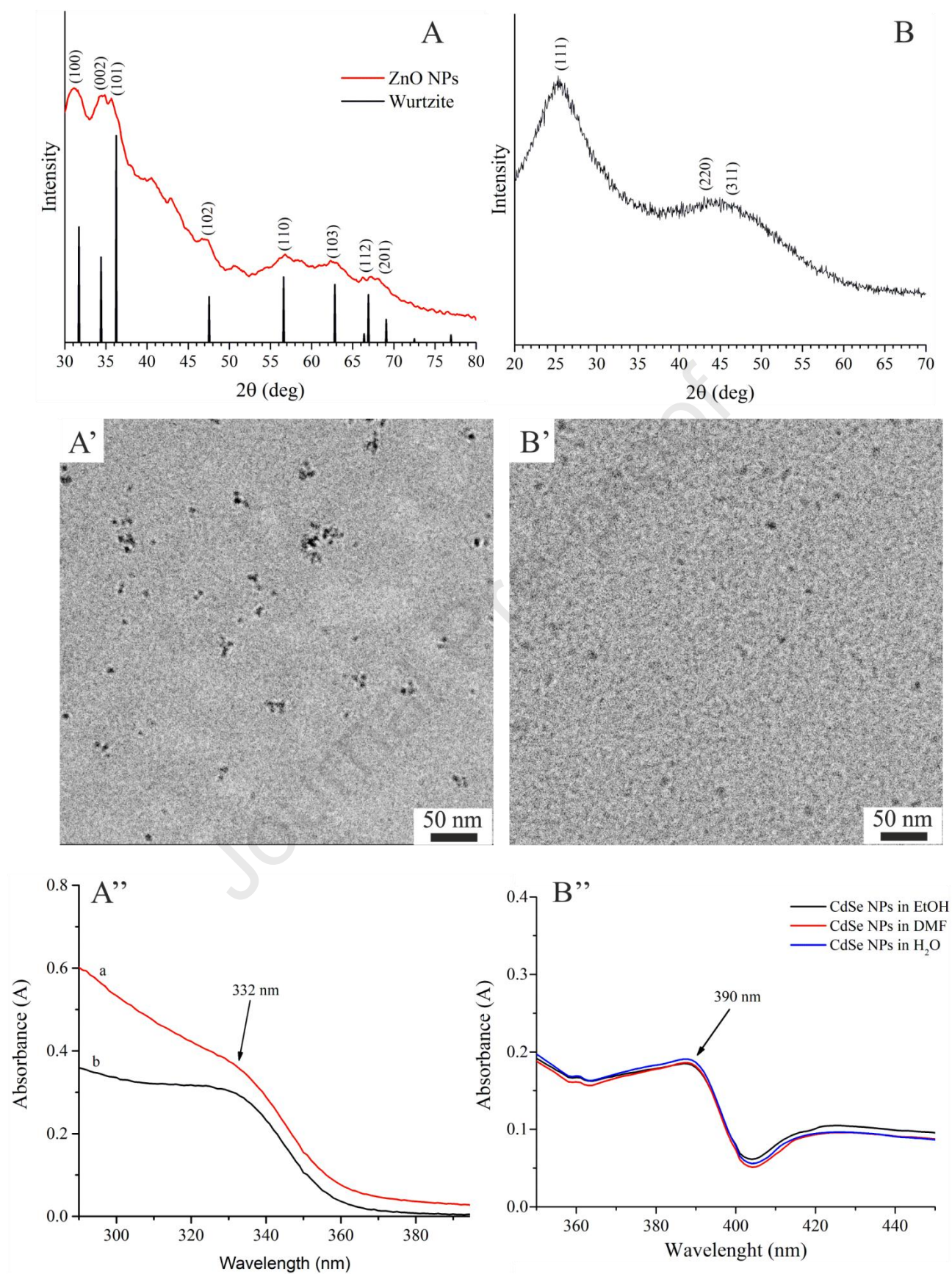
Figure 5. Wide angle X-ray powder diffraction (WAXS) profiles (A, B), TEM images (A', B') and UV-Vis absorption spectra in different solvents (A'', B'') of synthesized organic capped ZnO (A-
