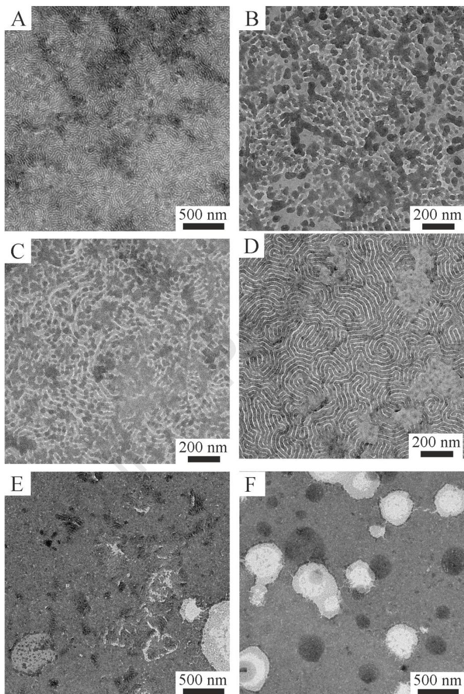
Figure 1. TEM images of PS- b -PMMA thin films, prepared by spin coating toluene solutions of 1 wt% BCP onto FSM6-ITO supports and annealed at 190 °C for 24 hours, after different UV irradiation times of 0 (A), 15 (B), 45 (C), 60 (D), 90 (E) and 120 (F) min and washing with acetic acid. Staining with RuO 4 was performed before TEM observation.
