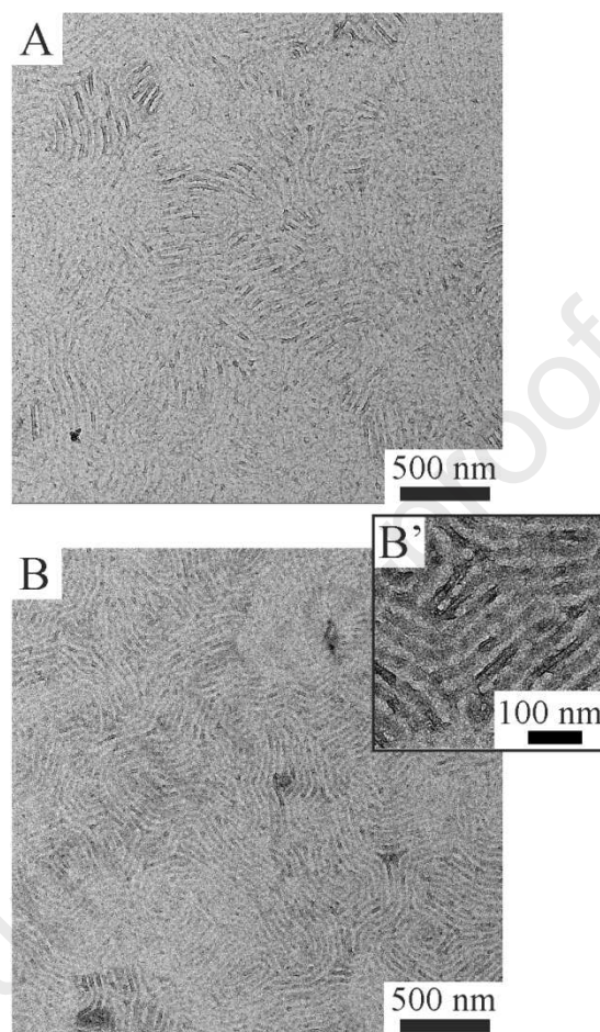
Figure 7. TEM images of nanoporous/nanocomposite thin films obtained by dipping the BCP-based nanoporous thin film in the CdSe NPs ethanol dispersion before (A) and after (B, B') RuO 4 staining of the PS domain. Six immersion/reemergence cycles and a sample/NPs dispersion contact time for each cycle equal to 150 s were used.
