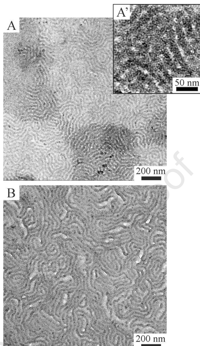
Figure 6. Bright-field TEM images of thin films prepared by spin-coating toluene solutions containing PS- b -PMMA BCP and ZnO NPs onto FSM6-ITO supports, and annealed at 190 °C for 24 hours, before (A, A') and after (B) UV treatment. The image A and A' were acquired after RuO 4 staining; no staining procedure, instead, was performed onto the UV-treated sample (B).
