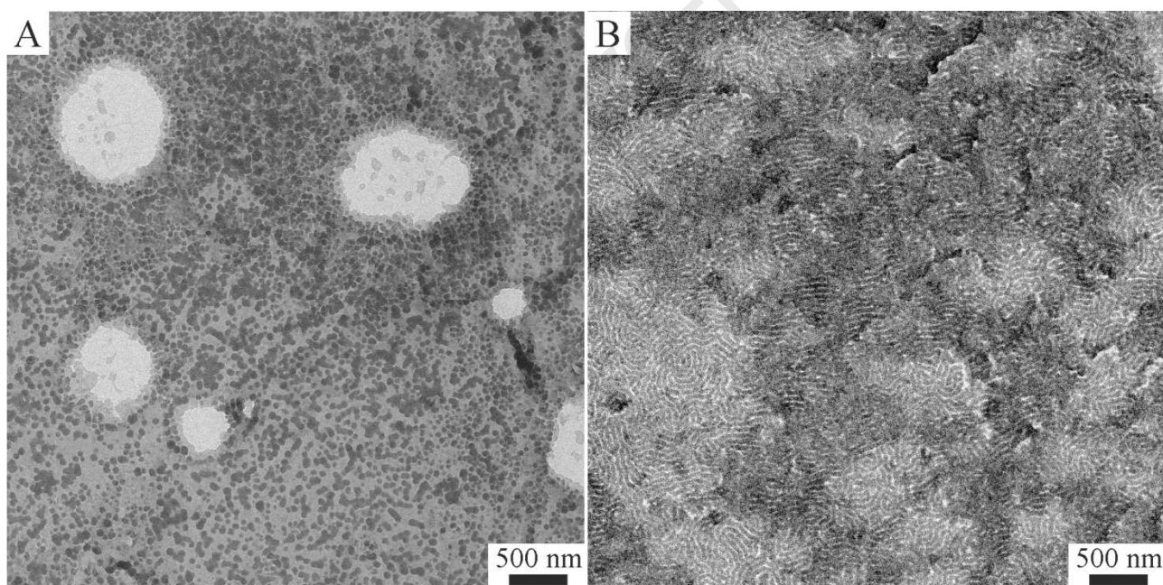
Figure 4. TEM images obtained after immersion in toluene for 120 minutes of the 15 min (A) and 60 min (B) UV-irradiated PS- b -PMMA thin films, prepared by spin coating toluene solutions of 1 wt% BCP onto FSM6-ITO supports and annealed at 190 °C for 24 hours. Staining with RuO 4 was performed before TEM observation.
