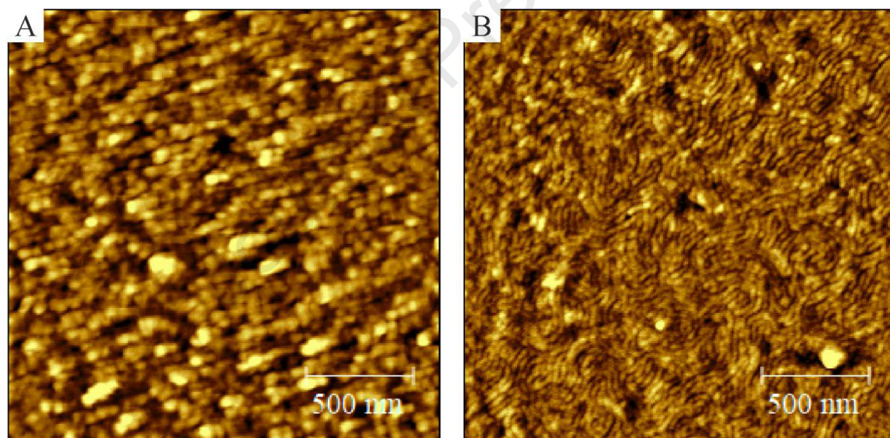
Figure S2. AFM height images of PS- b -PMMA thin films, prepared by spin coating toluene solutions of 1 wt% BCP onto ITO-FSM6 supports after thermal annealing at 190 °C for 24 hours, after (A) 15 and (B) 45 min of UV irradiation.
