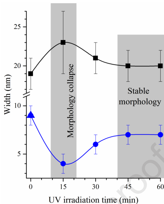
Figure 2. Size of the PS nanodomains (black squares) and of nanochannels (blue circles) left free upon removal of PMMA blocks present at time zero (blue triangle). Nanochannels were obtained after UV irradiation of PS- b -PMMA thin films, prepared by spin coating toluene solutions of 1 wt% BCP onto FSM6-ITO supports and annealed at 190 °C for 24 hours, for different times (15, 30, 45 and 60 min).
