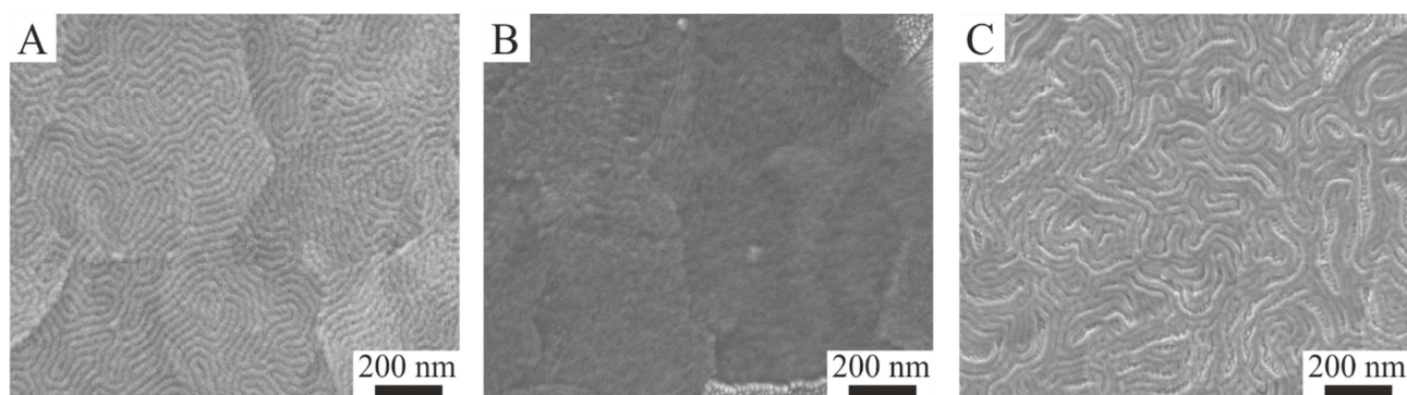
Figure S1. SEM images of PS- b -PMMA thin films, prepared by spin coating toluene solutions of 1 wt% BCP onto FSM6-ITO supports and annealed at 190 °C for 24 hours, before (A) and after 15 (B) and 60 (C) minutes of UV irradiation.
