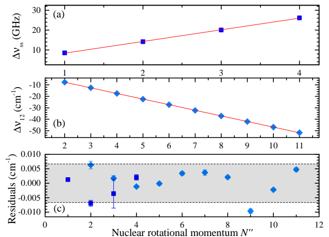
FIG. 8. Ground-state (a) spin splitting and (b) P -branch line splitting measurement with low- N levels of the B-X(0,0) band. (c) Combined fit residuals. The gray area represents the 200 MHz wavenumber uncertainty.
