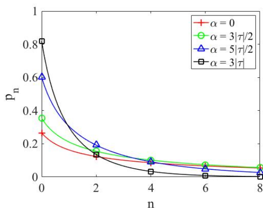
Figure 3. The even probability distribution (23) for |\tau| = 2 .
