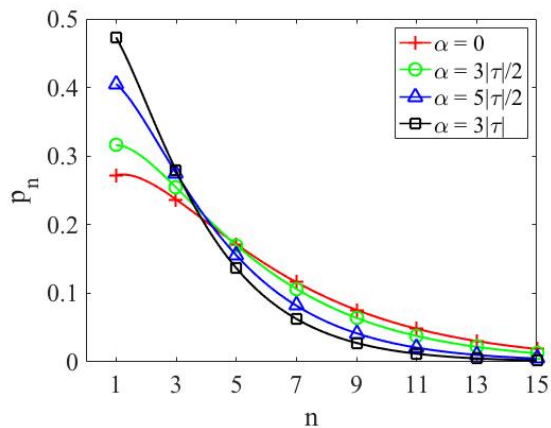
Figure 4. The odd probability distribution (24) for |\tau| = 1 .
