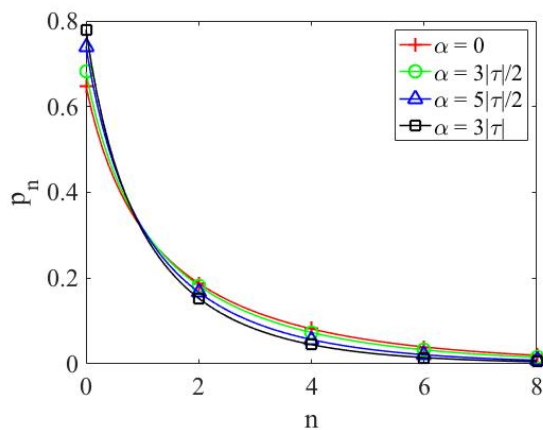
Figure 2. The even probability distribution (23) for |\tau| = 1 .
