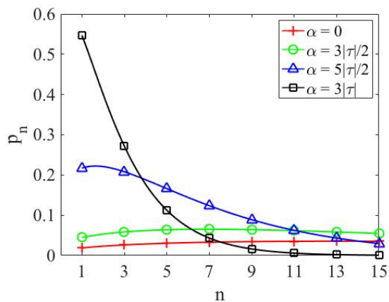
Figure 5. The odd probability distribution (24) for |\tau| = 2 .
