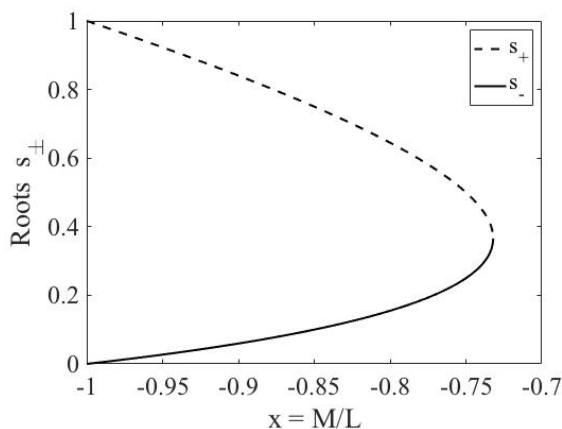
Figure 1. Squeezing transition curves corresponding to roots (22) of equation \mathcal{G}(s) = 0 . x is defined in [-1, 1 - \sqrt{3}] .
