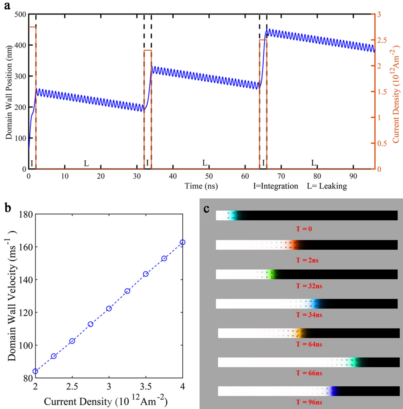
FIG. 4. Leaking and integration of the DW-MTJ neuron. (a) Time vs. DW position plot for three consecutive 2 ns long current pulses of magnitude 2.75, 2.3, and 2.5 \times 10^{12} \text{A/m}^2 , respectively, separated by 30 ns leaking periods. During the current pulse periods, integration functionality is taking place. The leaking functionality resulting from the magnetic field created by the fixed ferromagnet causes precessional DW motion. (b) Current density vs. DW velocity. (c) Mumax3 snapshots of the integration and leaking at the times noted by dashes in the plot of (a). (Multimedia view).
