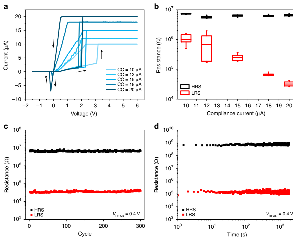
Fig. 4 DC operation modes of a single ZnO NW exhibiting multilevel memory capability. a I-V curves obtained by quasi-static DC voltage sweeps for different applied CC, showing bipolar resistive switching behaviour. b Measured LRS and HRS resistance values (read at 0.4 V) showing multilevel memory capability through the modulation of the programming current. Box plots were obtained from 15 consecutive cycles for each value of imposed CC on the same device. Midline represent median value, boxes the 25th and 75th percentiles and whiskers the 10th and 90th percentiles. c Endurance properties of the device acquired by full-sweep cycles with a programming current of 20 \mu\text{A} and d retention properties of a NW-based device after being switched to the LRS and HRS
