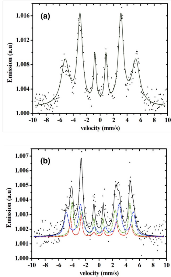
Fig. 4. Mössbauer spectrum of the \text{Fe}_{56}\text{Pd}_{44} thin film alloy (symbols: experimental data, lines: fits) (a) as-prepared and (b) annealed at 550\text{ }^{\circ}\text{C} for 60 min (ordered \text{L1}_0 FePd phase (green), twin boundaries (red), antiphase boundaries (blue), the \text{Fe}_{56}\text{Pd}_{44} thin film alloys (black)).
