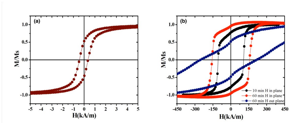
Fig. 5. Hysteresis loops for Fe_{56}Pd_{44} thin film: (a) as-deposited; (b) annealed at 550 °C for 10 minutes (black curve), 60 minutes in-plane (red curve) and out-of-plane (blue curve).
