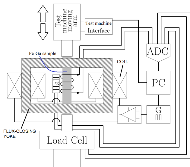
Fig. 2. Scheme of the experimental setup.
