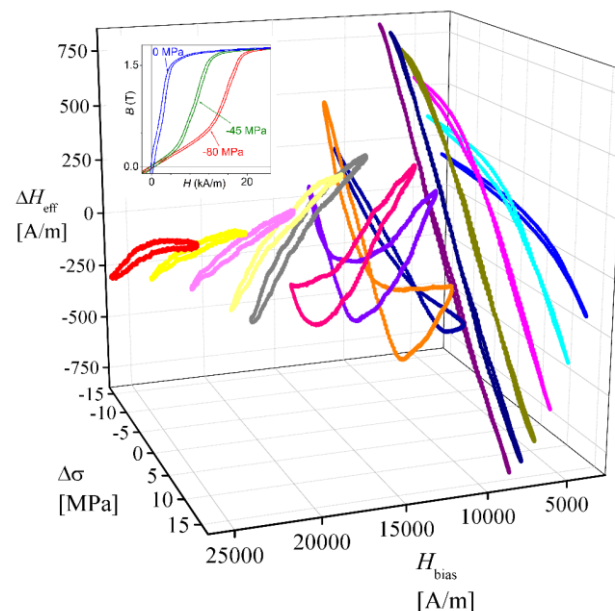
Fig. 4. Measured effective field variation \Delta H_{\text{eff}} versus dynamic stress \Delta\sigma at 20 Hz for different values of the applied field bias H_{\text{bias}} . Compressive pre-stress \sigma_{\text{bias}} = -45 \text{ MPa} , dynamic stress peak amplitude \Delta\sigma_{\text{max}} = \pm 15 \text{ MPa} . The inset shows examples of major (B, H) hysteresis loops measured with constant pre-stress \sigma_0 = 0, \sigma_0 = -45 \text{ MPa}; \sigma_0 = -80 \text{ MPa} .
