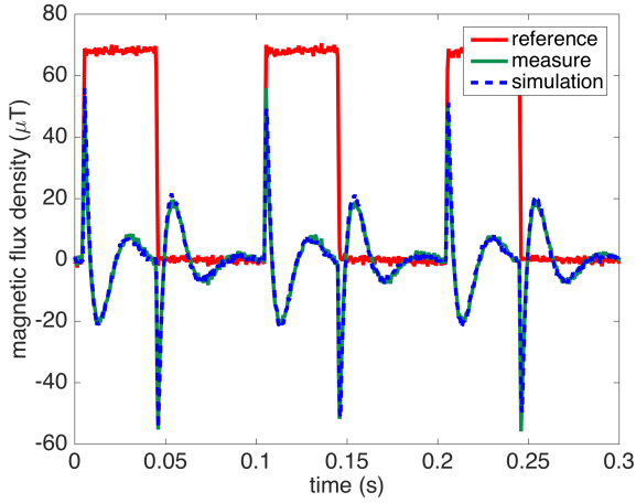
Fig. 8. Simulation of the measurement artefact related to f_{cut} = 30 Hz. The red curve is the reference waveform, the green curve is the waveform measured by the meter and the blue (dashed) curve is the simulation.
