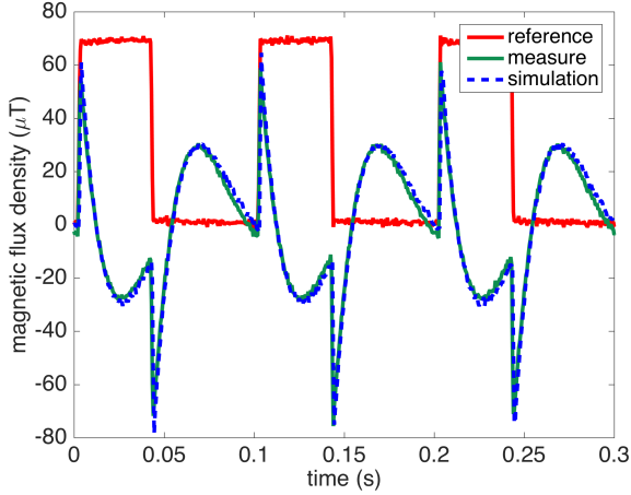
Fig. 7. Simulation of the measurement artefact related to f_{cut} = 10 Hz. The red curve is the reference waveform, the green curve is the waveform measured by the meter and the blue (dashed) curve is the simulation.
