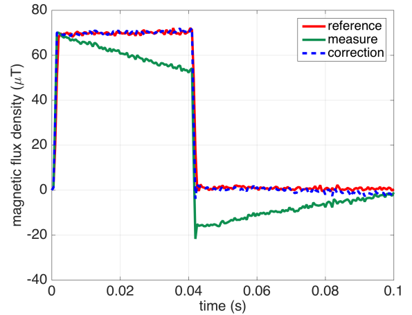
Fig. 9. Test of the correction procedure on the measured waveform with f_{cut} = 1 Hz. The red curve is the reference waveform, the green curve is the waveform measured by the meter and the blue (dashed) curve waveform obtained by means of the correction procedure.
